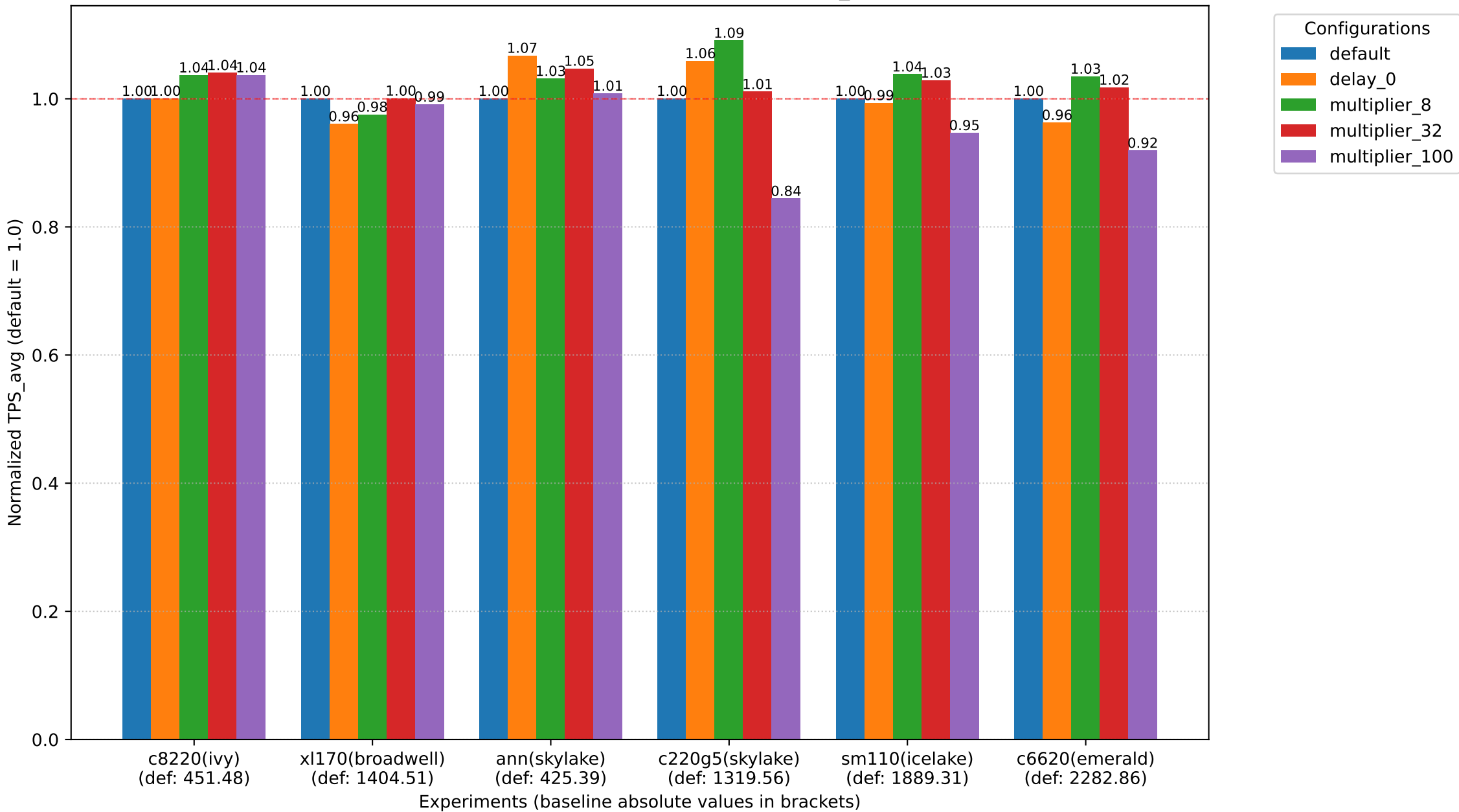
not consolidated sysbench 16threads - TPS_avg
