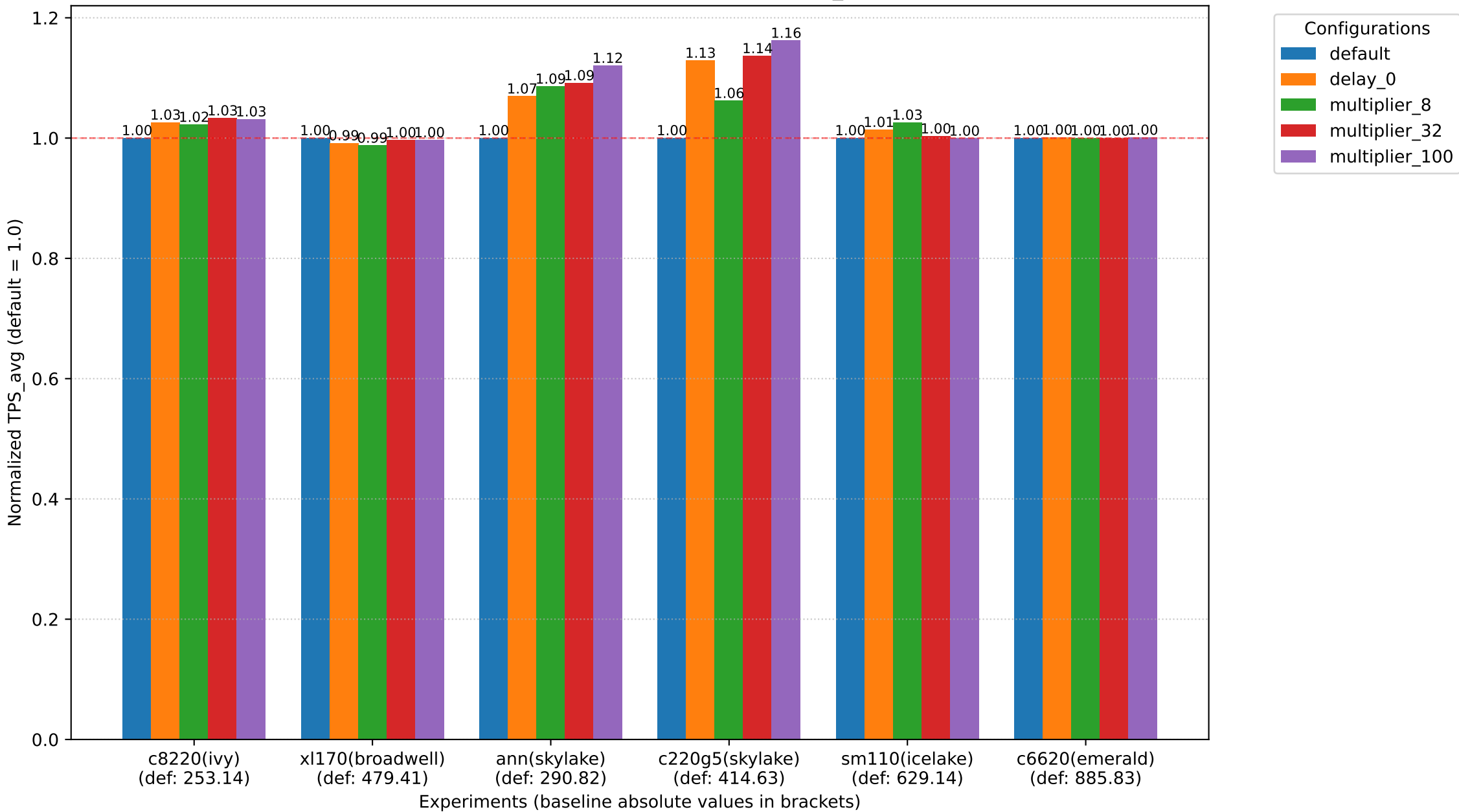
not consolidated sysbench 1threads - TPS_avg
