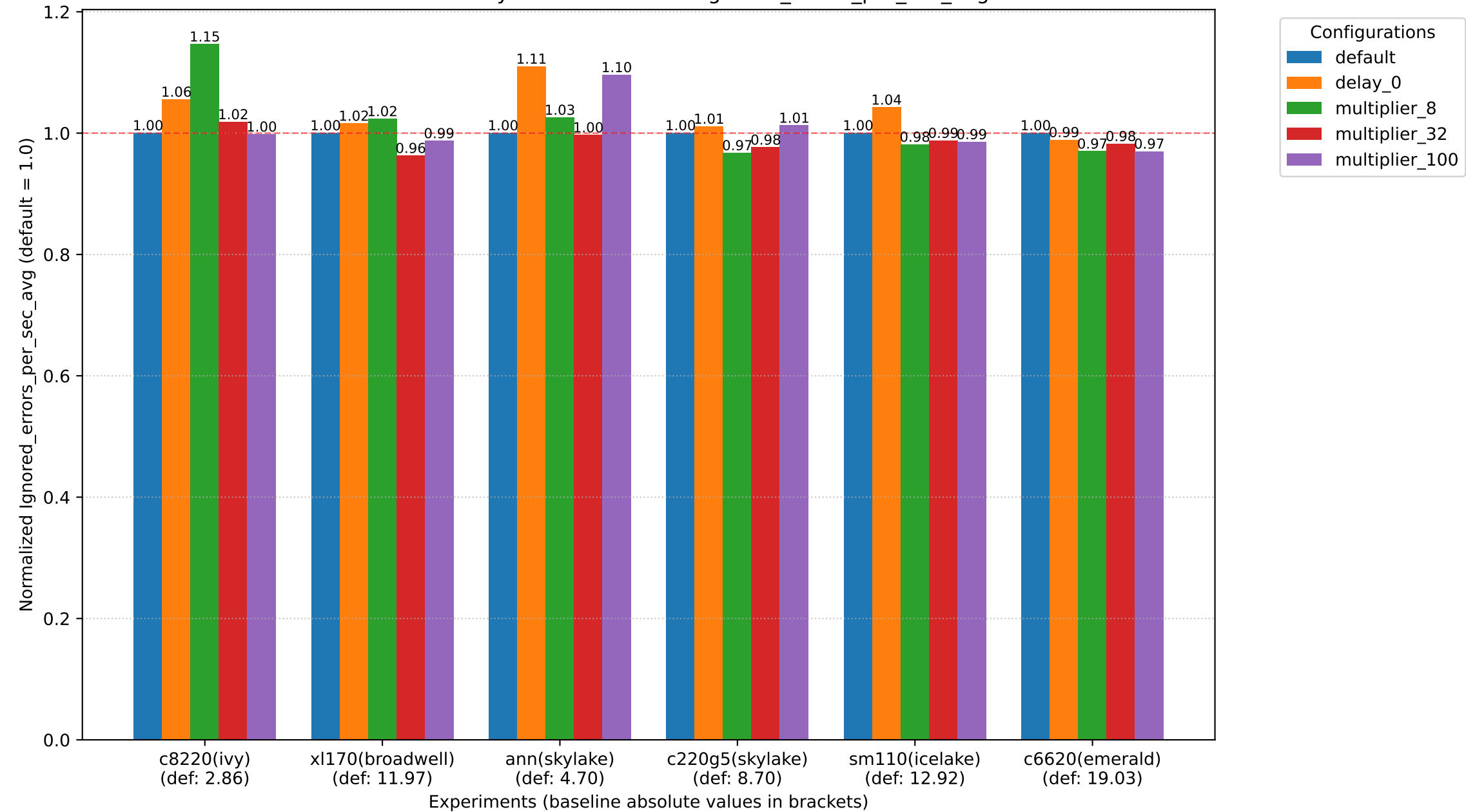
not consolidated sysbench 5threads - Ignored_errors_per_sec_avg
