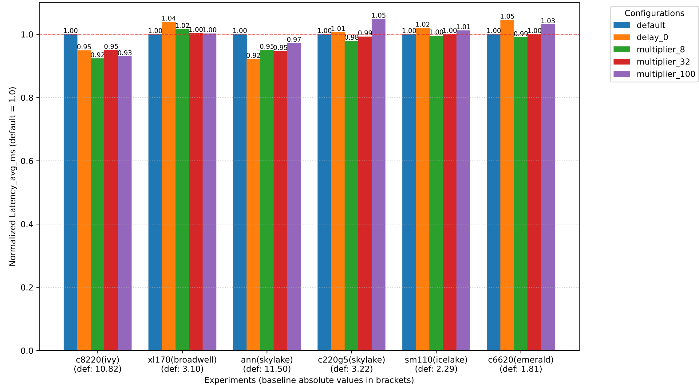
not consolidated sysbench 5threads - Latency_avg_ms
