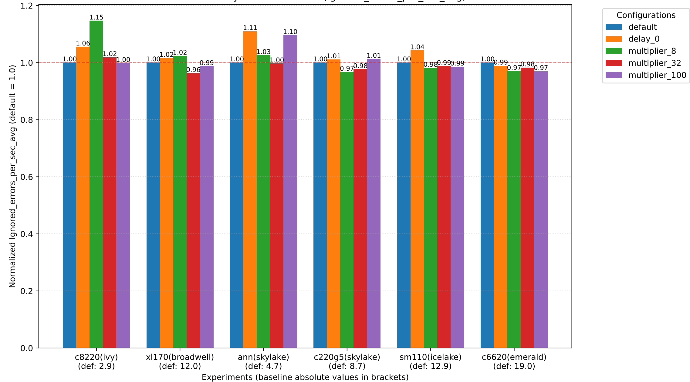
not consolidated sysbench 1tthreads (Ignored_errors_per_sec_avg)
