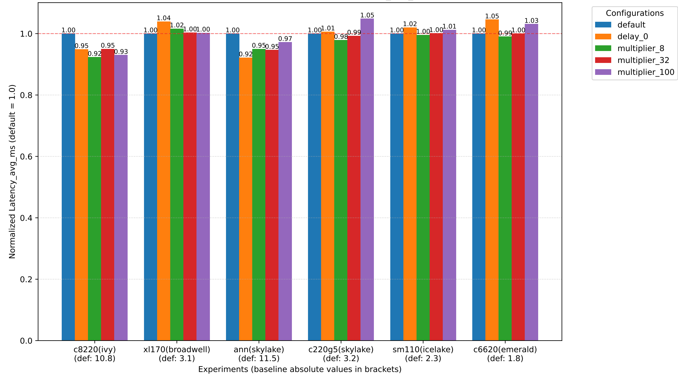
not consolidated sysbench 1threads (Latency_avg_ms)
