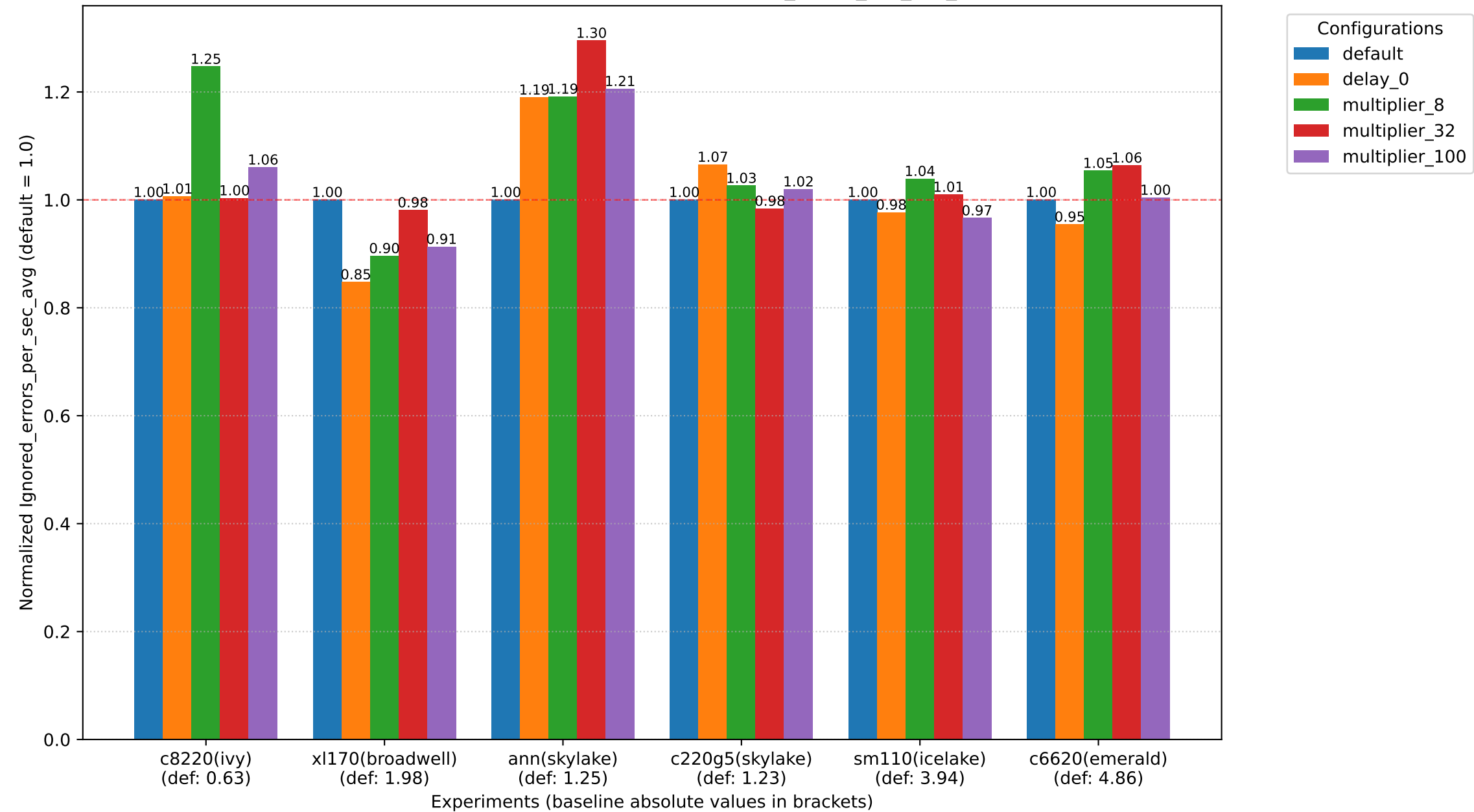
not consolidated sysbench 2threads - Ignored_errors_per_sec_avg
