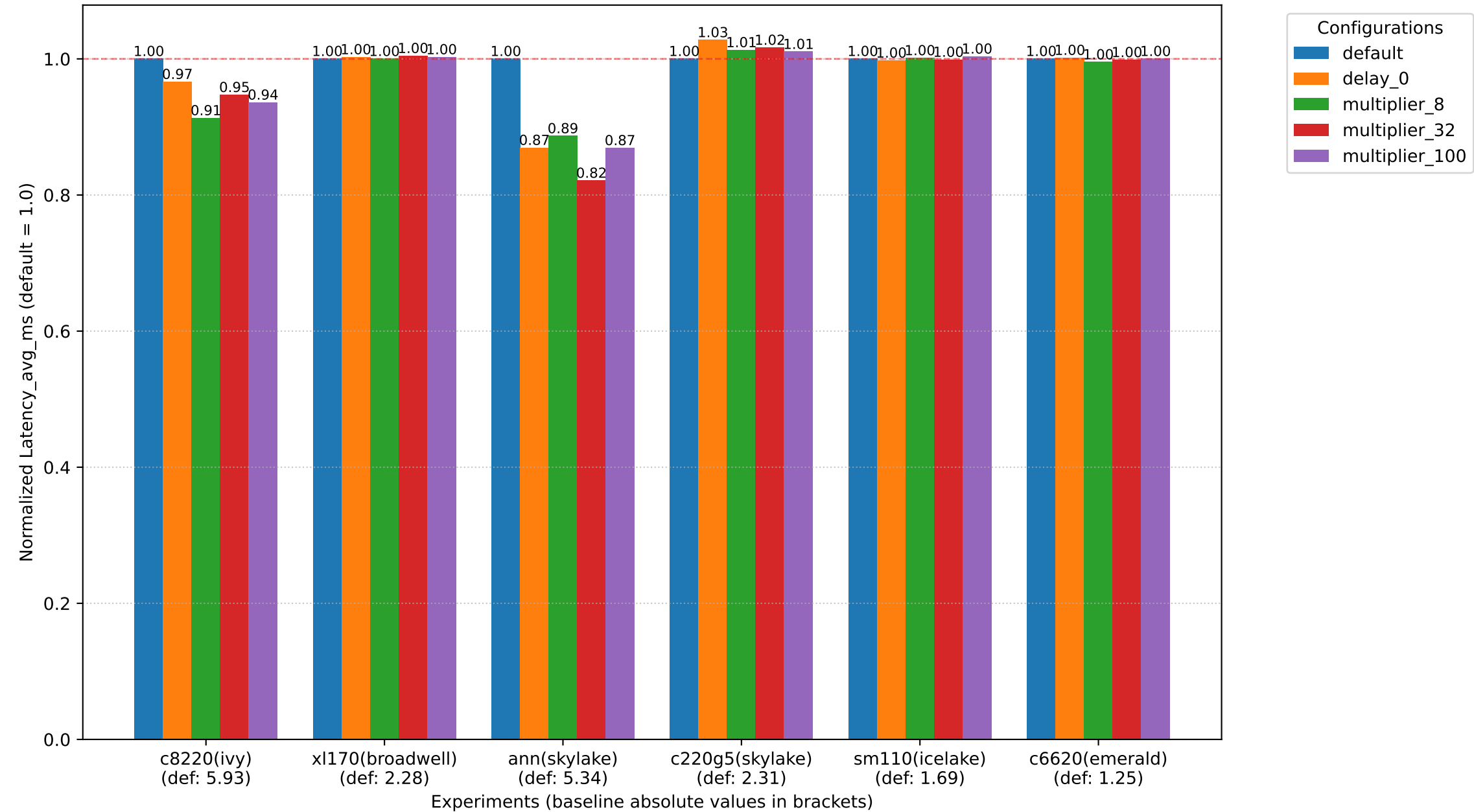
not consolidated sysbench 2threads - Latency_avg_ms
