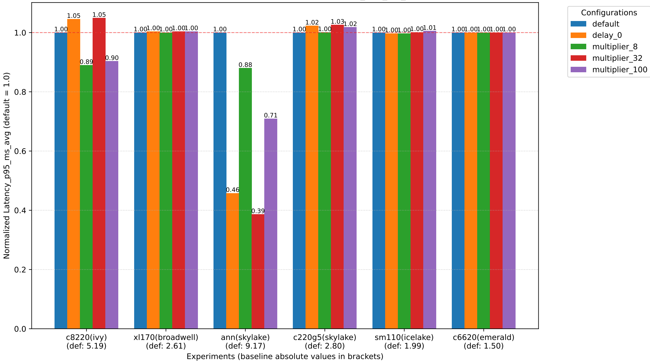
not consolidated sysbench 2threads - Latency_p95_ms_avg
