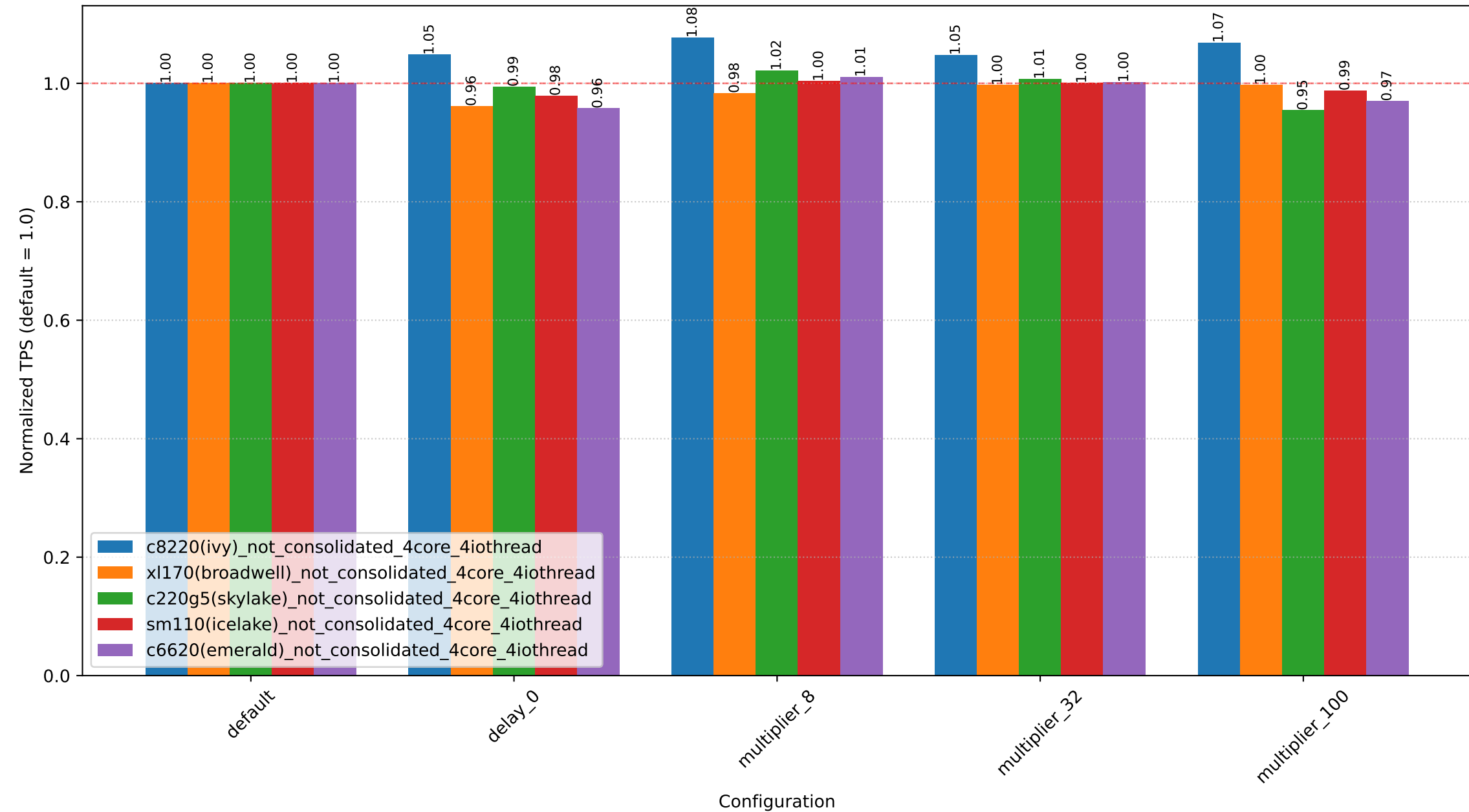
not consolidated sysbench 16threads
