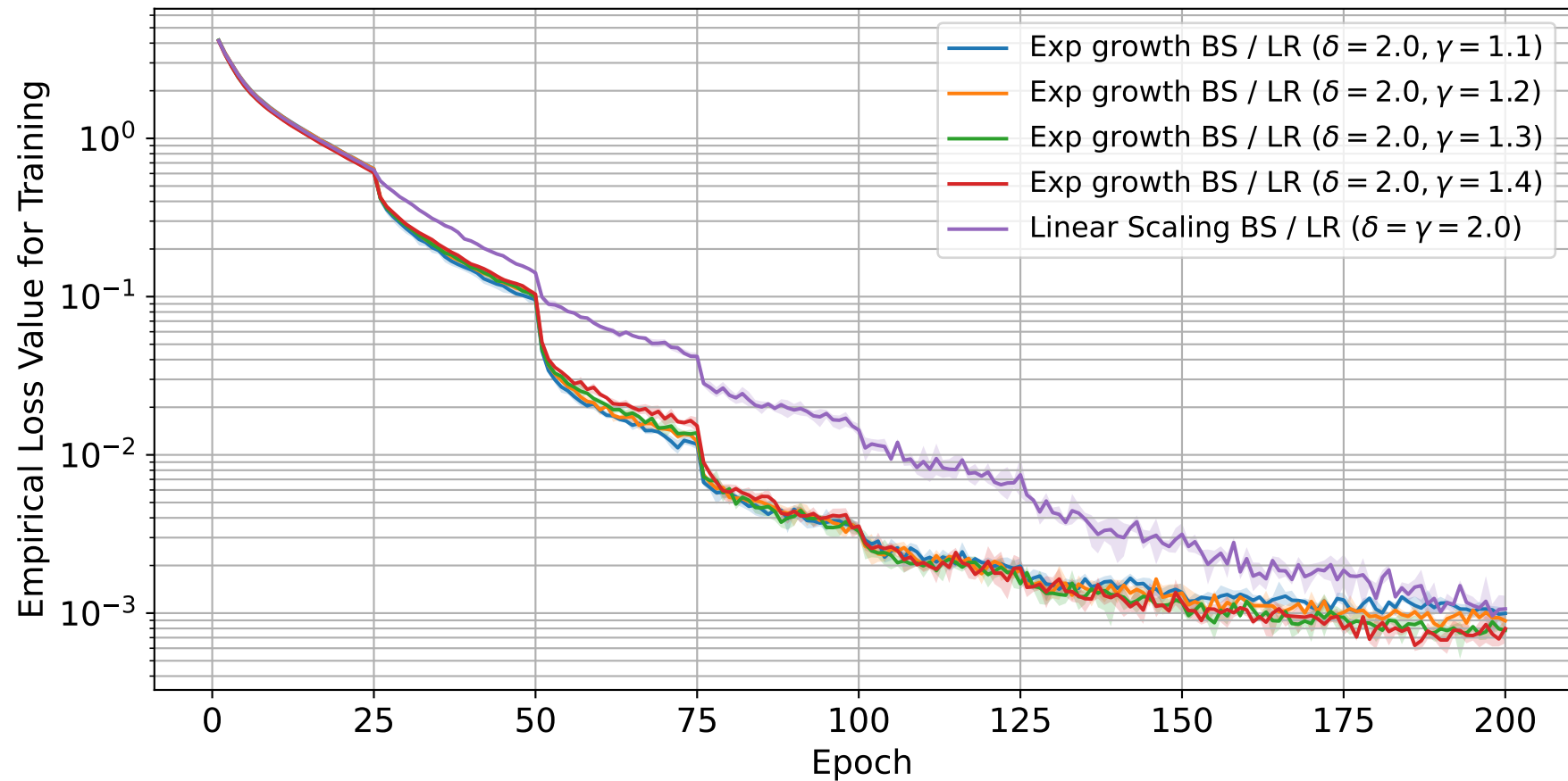
ResNet-18 on CIFAR-100
