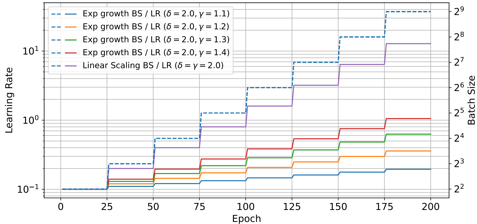
ResNet-18 on CIFAR-100
