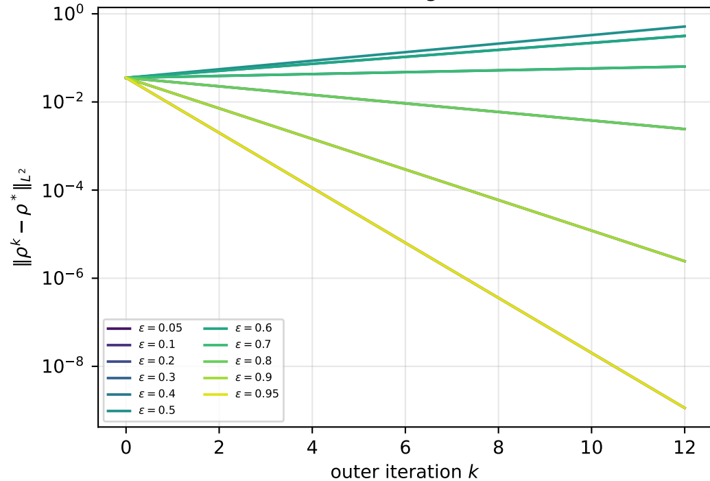
MFG-LWR convergence curves
