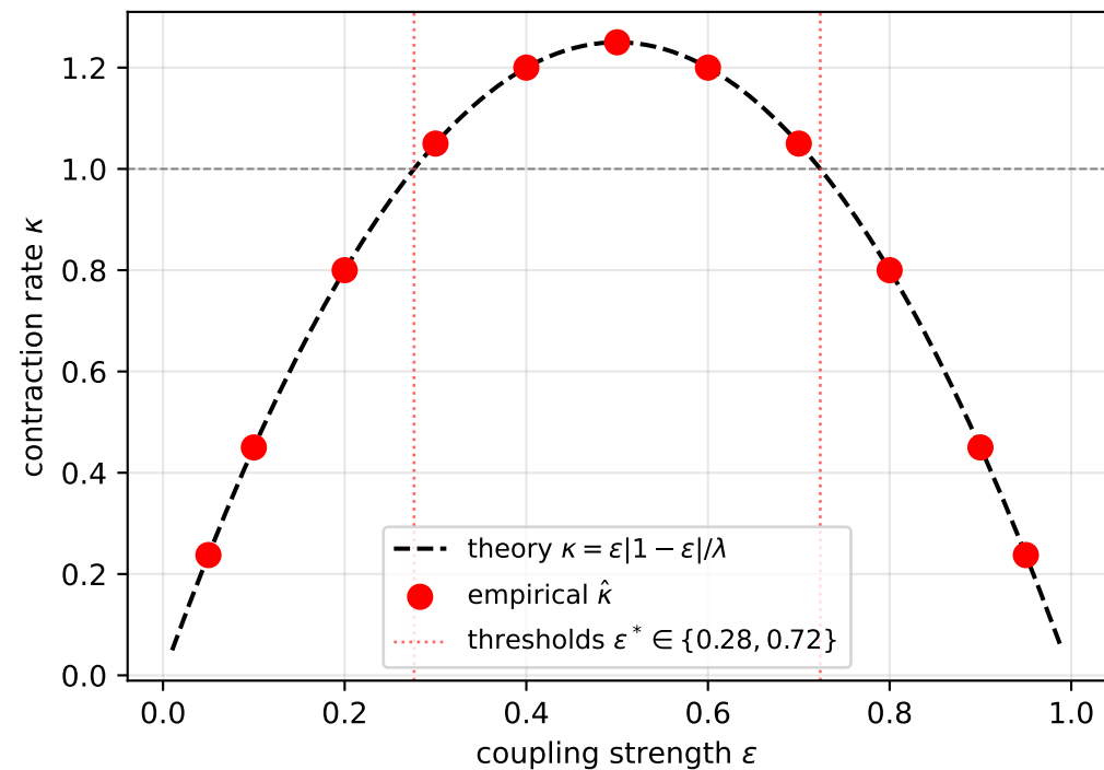
Bilinear R = \rho p , \lambda = 0.2
