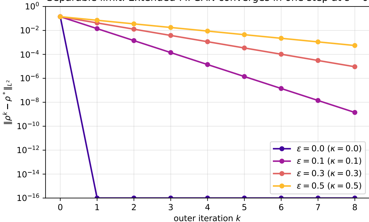
Separable limit: Extended-MFGAN converges in one step at \varepsilon = 0
