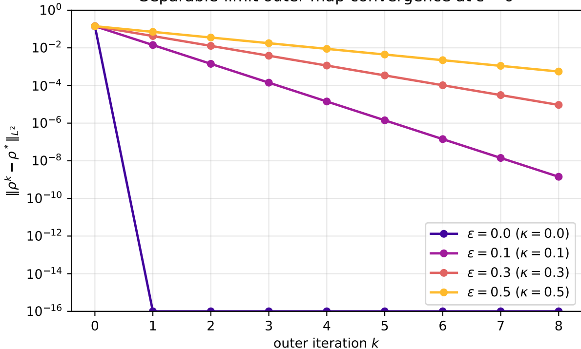
Separable-limit outer-map convergence at \varepsilon = 0
