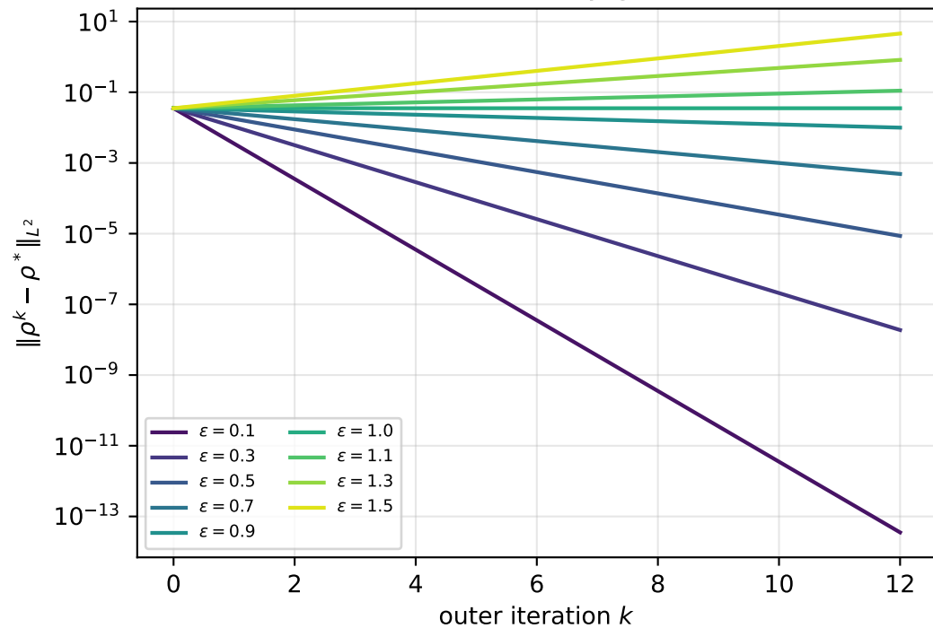
Geometric decay/growth
