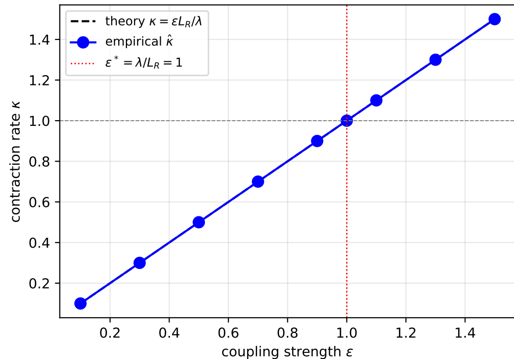
Phase transition at \varepsilon^* = 1
