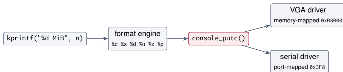
Figure 2: Output path. Adding a third sink later (a log buffer for dmesg ) is one line.
