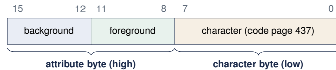
Figure 1: One 16-bit VGA text cell. White on blue is attribute 0x1F ; the cell for “A” is then 0x1F41 .
