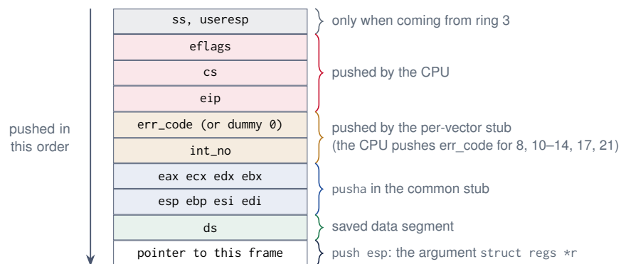
Figure 3: The stack when isr_handler is called. struct regs lists these fields from the bottom (ds) up.
