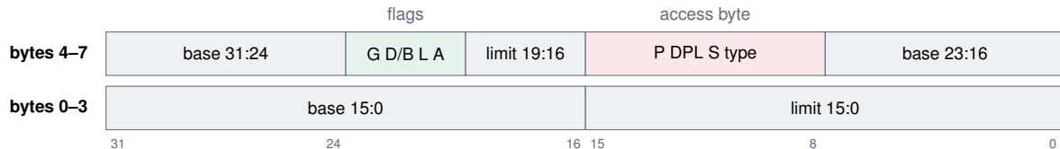
Figure 2: The 8-byte segment descriptor. Base and limit are scattered across both halves.
