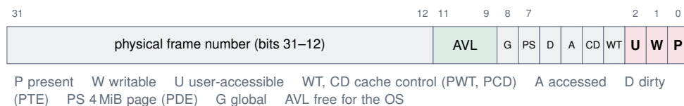
Figure 2: The format of a page directory or page table entry.
