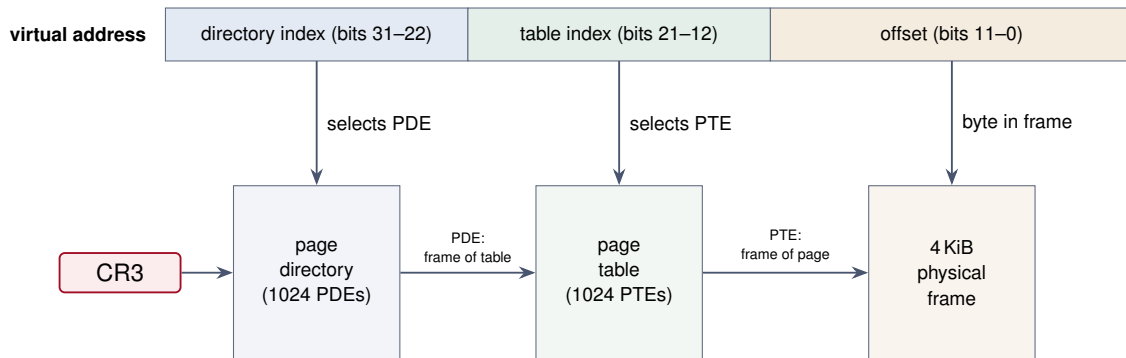
Figure 1: How the MMU translates a 32-bit virtual address with 4 KiB pages. Every pointer in these tables is a physical address.
