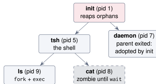
Figure 1: A Turk-OS process tree in Phase 14. Every process except init has a parent that must eventually wait for it.
