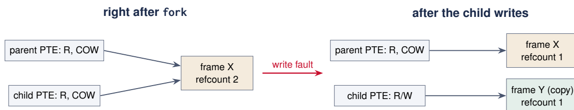
Figure 2: Copy-on-write for one page. The parent's next write finds refcount 1 and only needs its PTE made writable.
