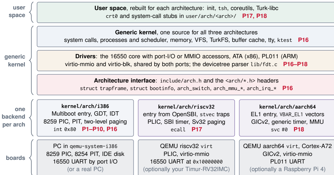
Figure 4: Turk-OS 2.0 after Stage V: one generic kernel, one architecture interface, three backends and three boards.
