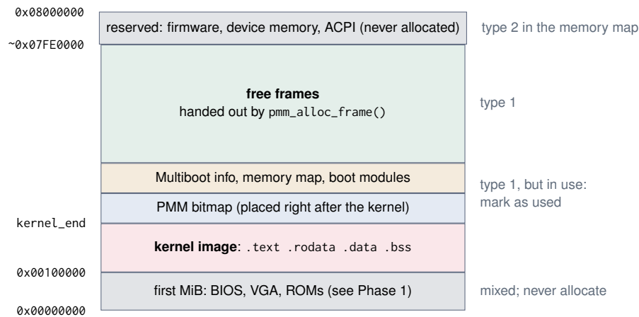
Figure 1: Physical memory of a 128 MiB QEMU machine (not to scale). Only frames in the green area are free.
