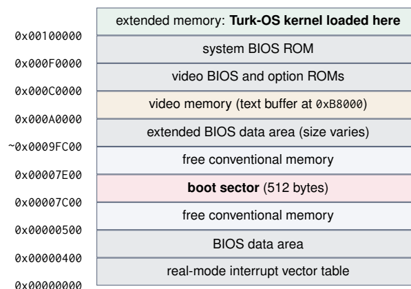
Figure 4: The first megabyte of a PC's physical memory (not to scale). Addresses mark the bottom of each region.
