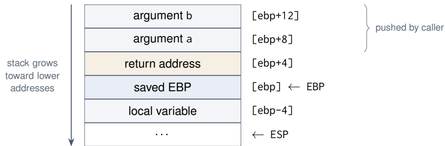
Figure 2: Stack frame inside f(a, b) after push ebp; mov ebp, esp . Higher addresses are at the top.
