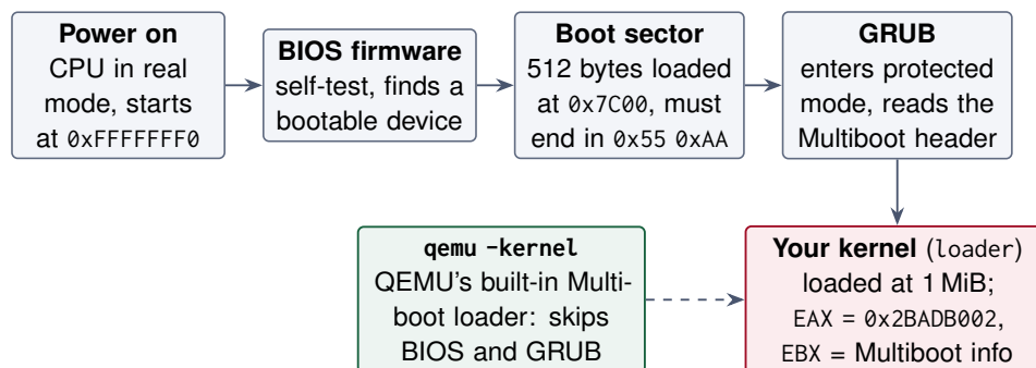
Figure 3: From power-on to the kernel. In Task 1.3 you replace the boot sector with your own; from Task 1.4 on GRUB (or QEMU) does it.
