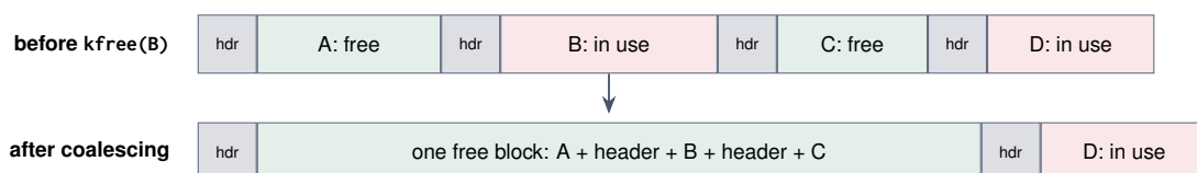
Figure 1: Freeing B between two free neighbours merges all three into a single block. Without coalescing, a request larger than A, B or C alone would fail.
