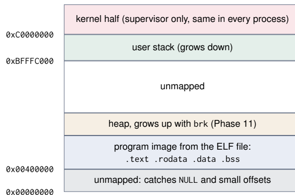
Figure 2: The address space of a Turk-OS user process.
