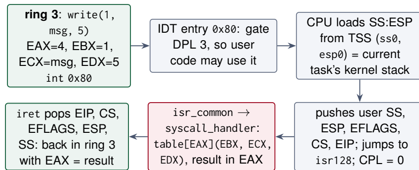
Figure 1: The round trip of a system call.
