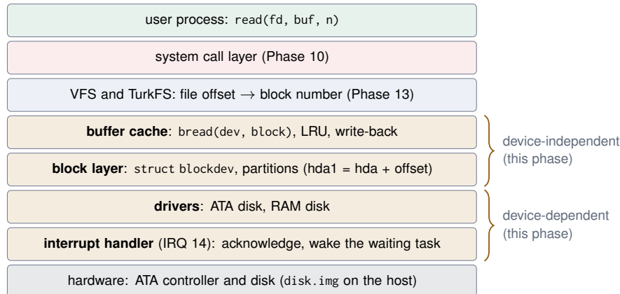
Figure 1: The storage stack. A read on a file passes through every layer; a cache hit stops at the buffer cache.
