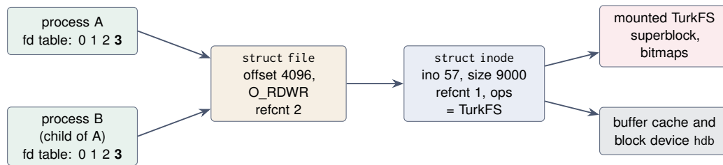
Figure 1: After fork, descriptor 3 in both processes refers to the same open file, and so to the same offset.
