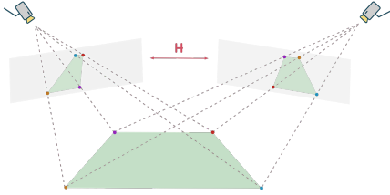
Figure 2: Homography Estimation
