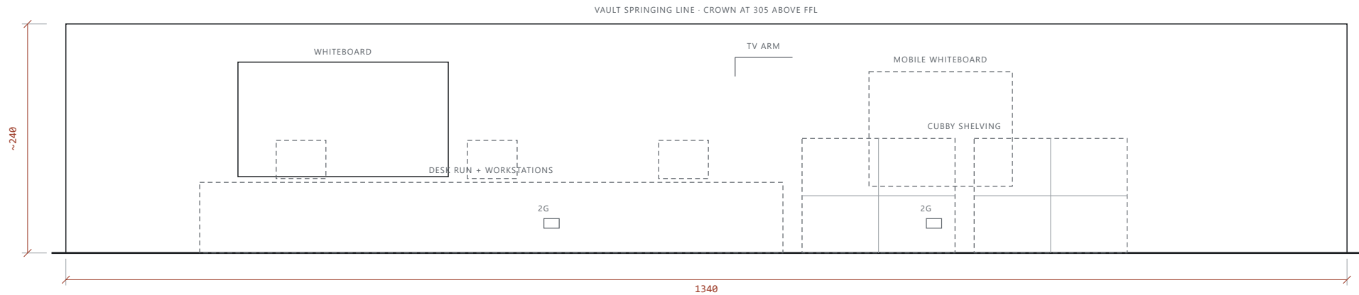
ELEVATION S · NORTH WALL PAINTED PLASTER · WHITEBOARD · DESK RUN
