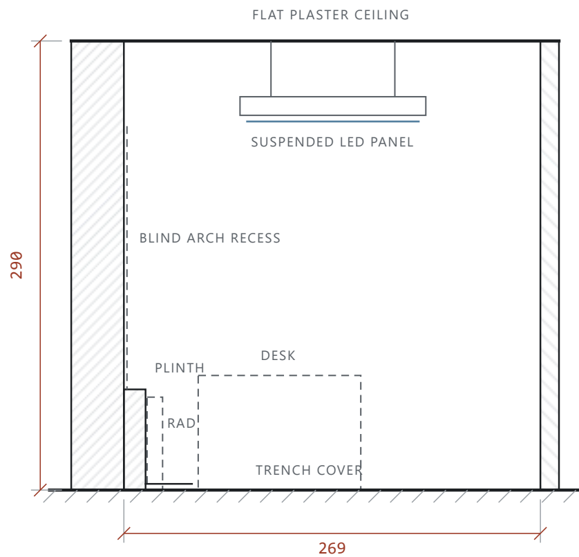
SECTION B-B LOOKING EAST · CUT AT x = 380
