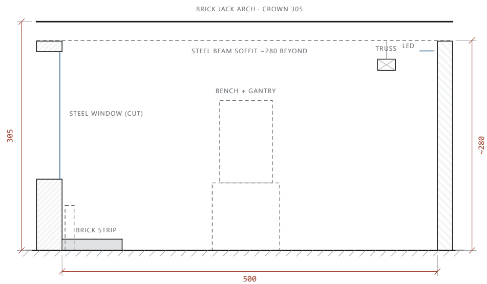
SECTION C-C LOOKING EAST
