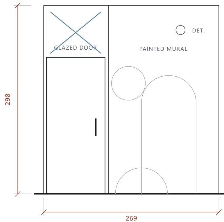
ELEVATION H · WEST END PAINTED MURAL · GLAZED SCREEN + DOOR AT SOUTH
