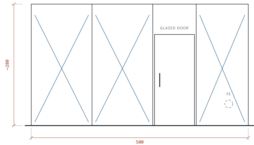
ELEVATION Q · EAST END GLAZED SCREEN + DOOR TO CORRIDOR
