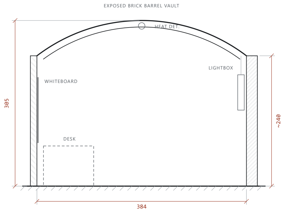
SECTION D-D LOOKING EAST
