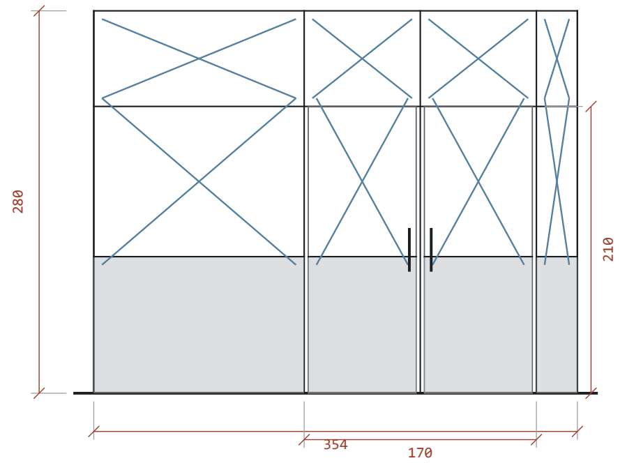
ELEVATION C GLAZED STEEL PARTITION + DOUBLE DOORS
