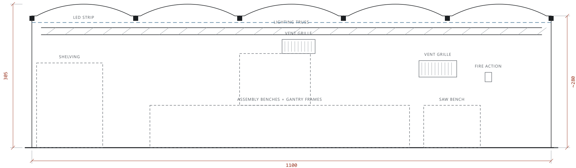
ELEVATION P · SOUTH WALL POLISHED PLASTER · SUSPENDED LIGHTING TRUSS + LED STRIP
