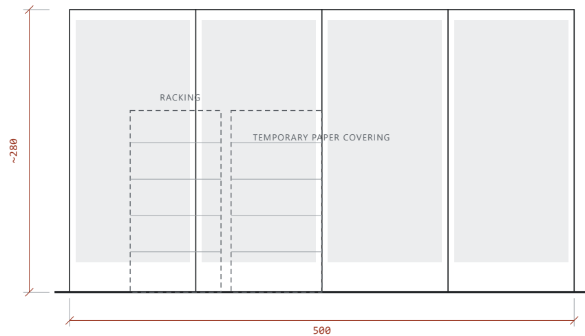
ELEVATION R · WEST END GLAZED SCREEN · PAPERED OVER · KITCHEN BEYOND
