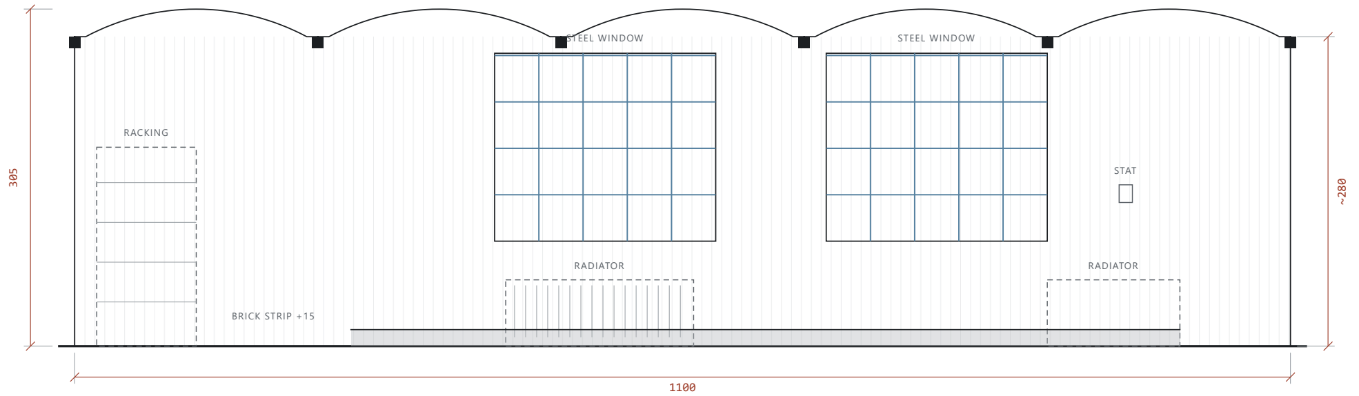
ELEVATION N · NORTH WALL EXPOSED BRICK · STEEL WINDOWS · RAISED BRICK STRIP AT BASE
