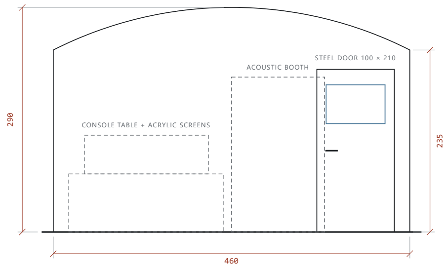
ELEVATION G · EAST END PLASTERED WALL · STEEL DOOR
