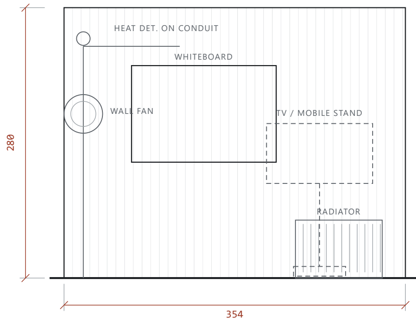
ELEVATION A EXPOSED BRICK WALL
