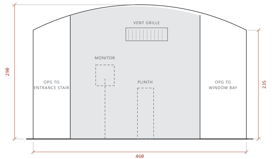
ELEVATION H · WEST END GREEN PARTITION · OPEN BOTH SIDES
