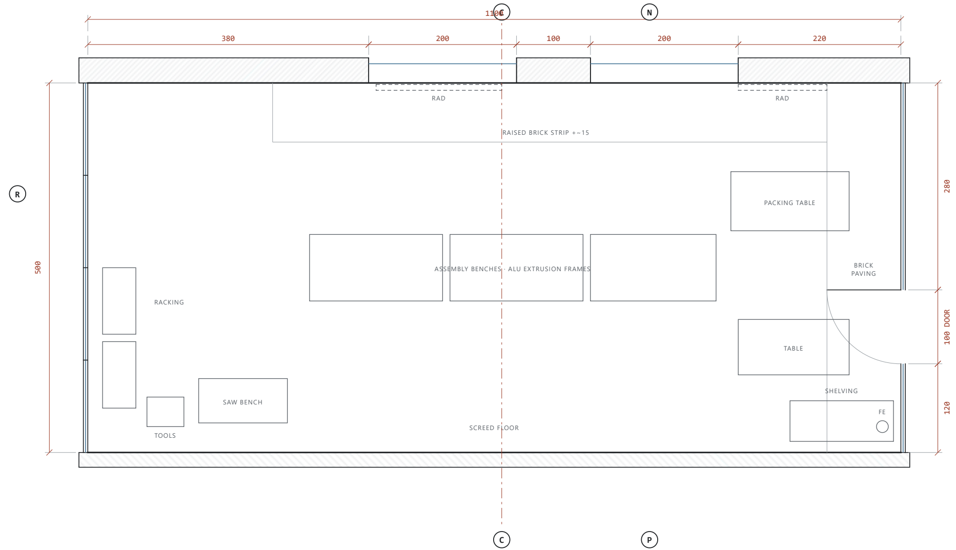
FLOOR PLAN · ENGINEERING
