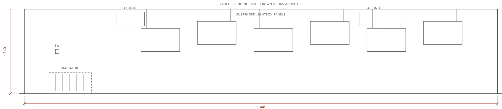
ELEVATION T · SOUTH WALL POLISHED PLASTER · SUSPENDED LIGHTBOX ROW · AC UNITS
