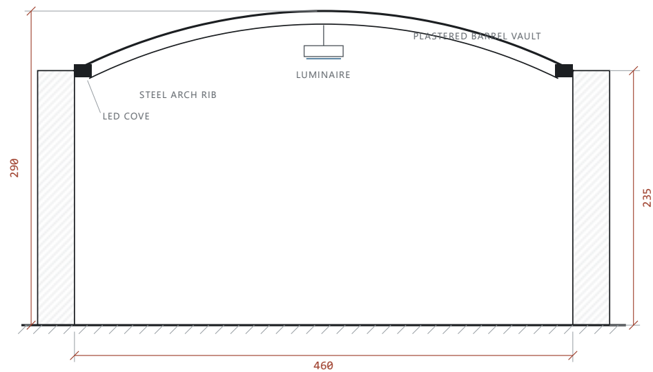
SECTION A-A LOOKING EAST
