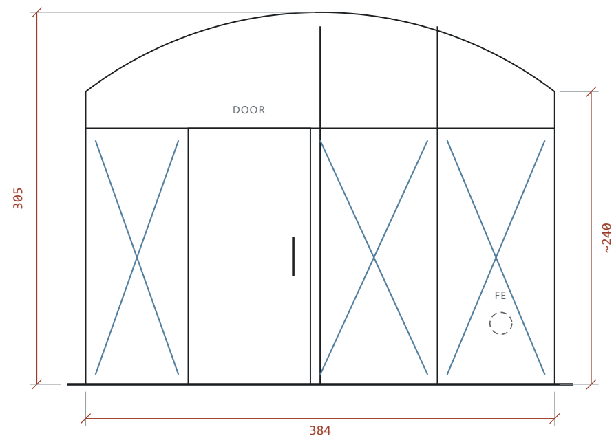
ELEVATION U · WEST END EXTERNAL STEEL GLAZED SCREEN + DOOR
