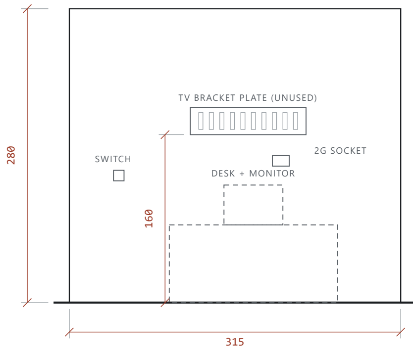
ELEVATION D PAINTED PARTITION WALL
