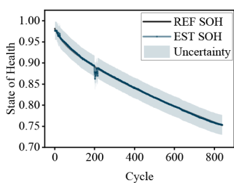
(a) MRVR
