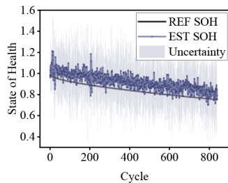
(c) BMNN
