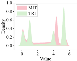
(a) KDE curve of current signals
