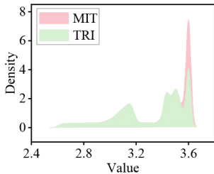
(b) KDE curve of voltage signals
