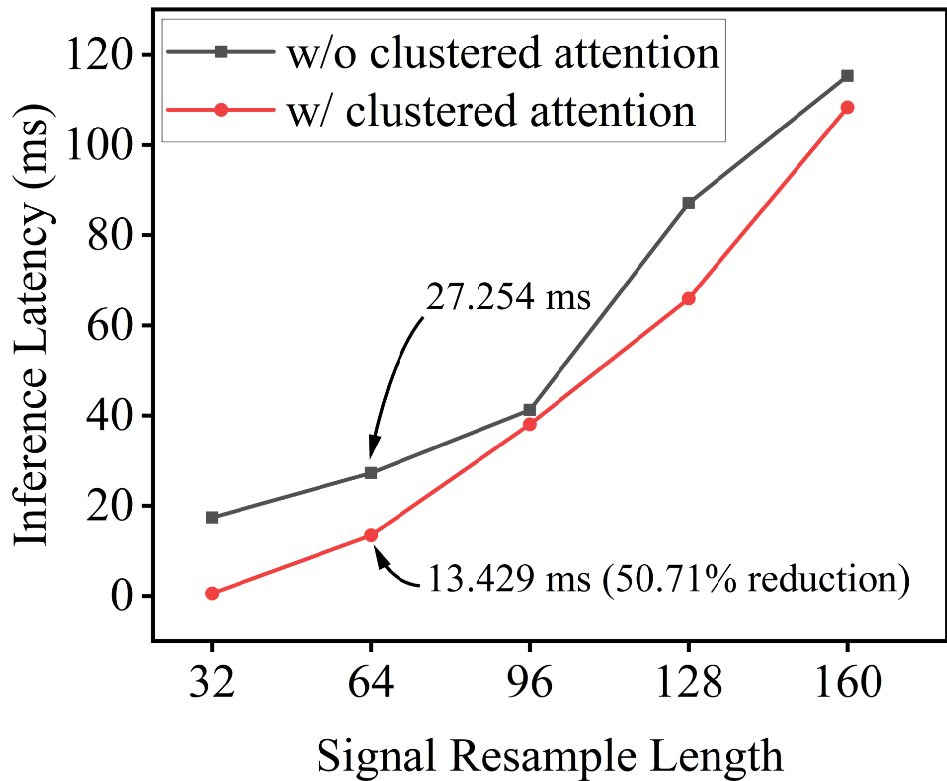
(a) Inference latency with and without clustered attention
