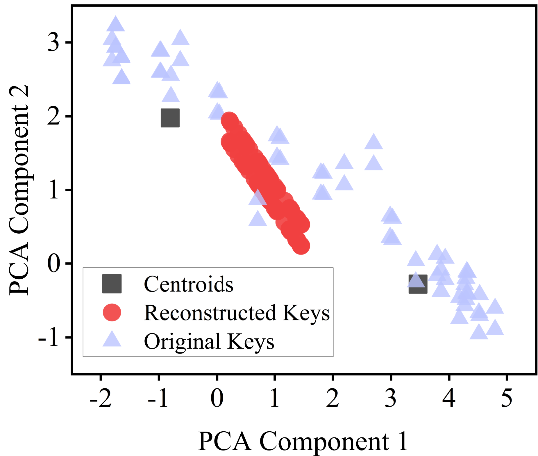
(b) Visualization of attention key sparsification
