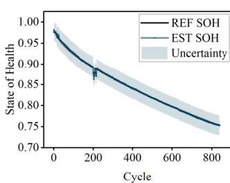
(a) MRVR
