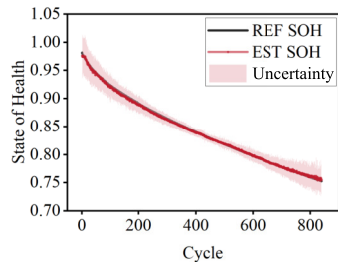
(h) HSSTT
