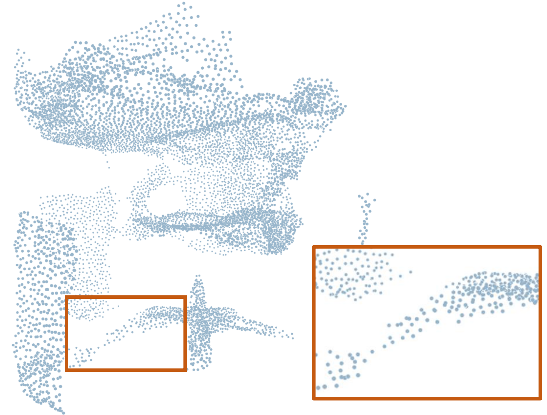
PU-GAN
