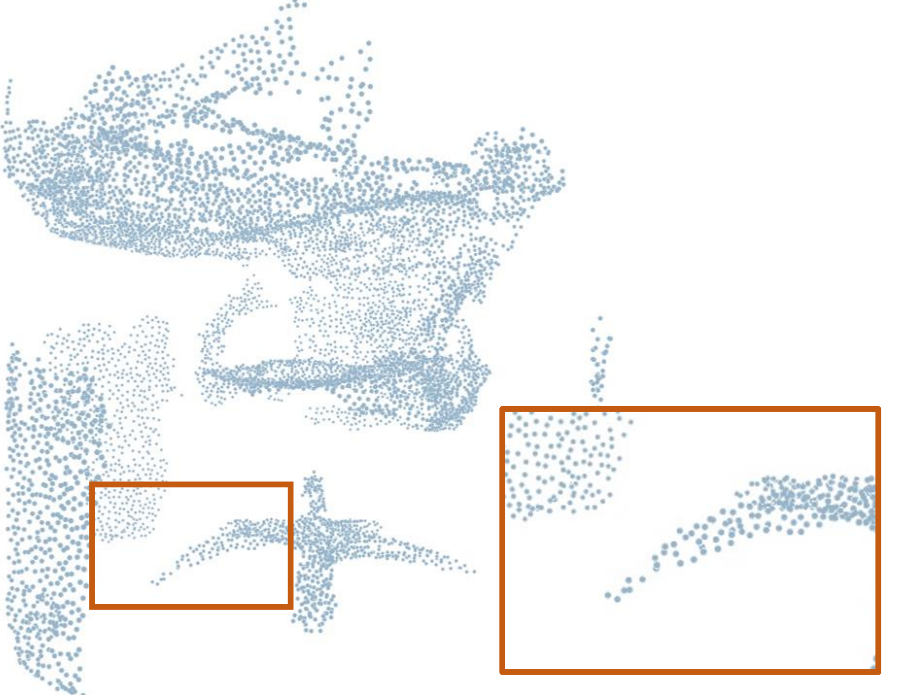
PU-Transformer
