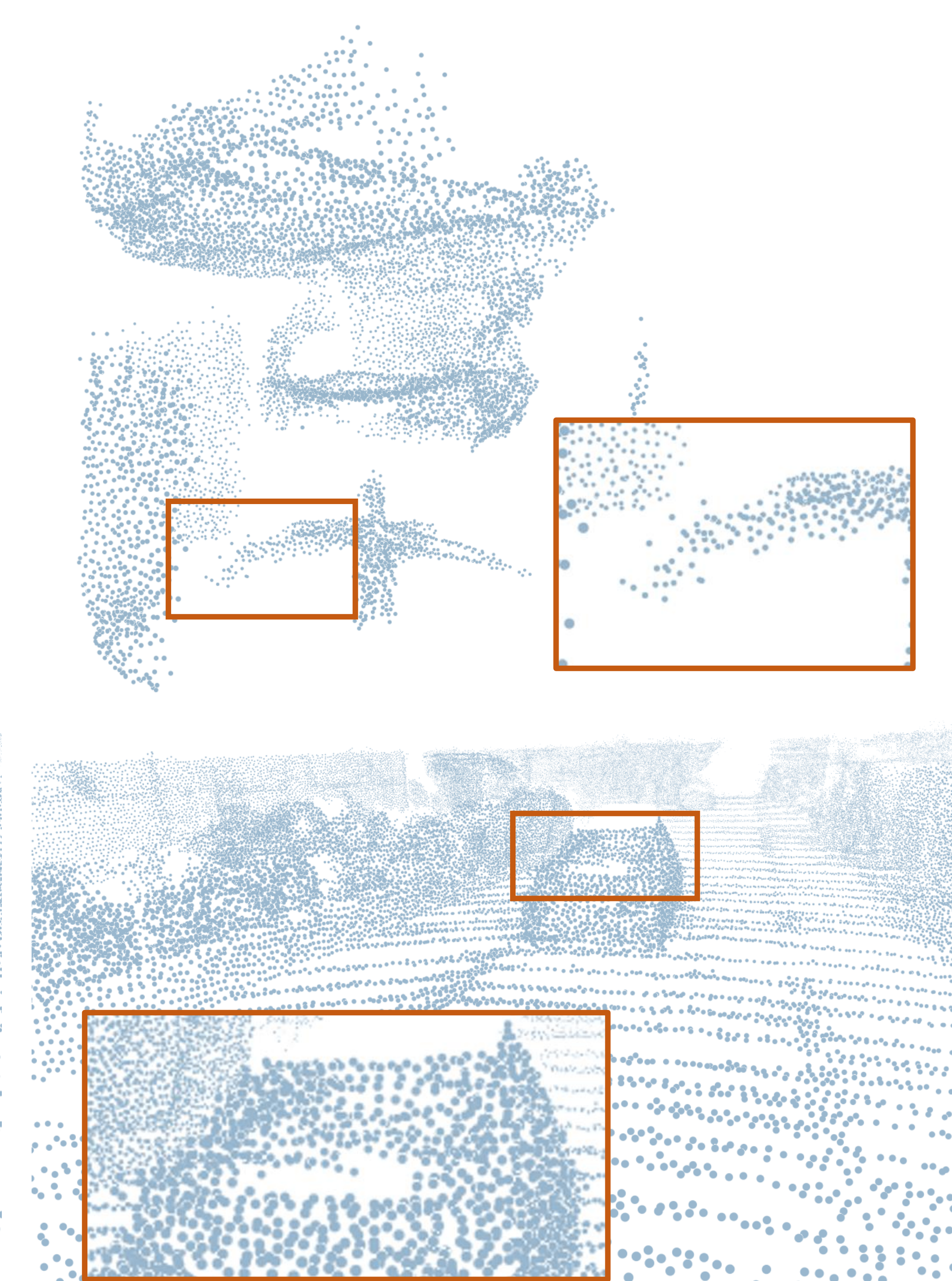
(c) PU-GCN
