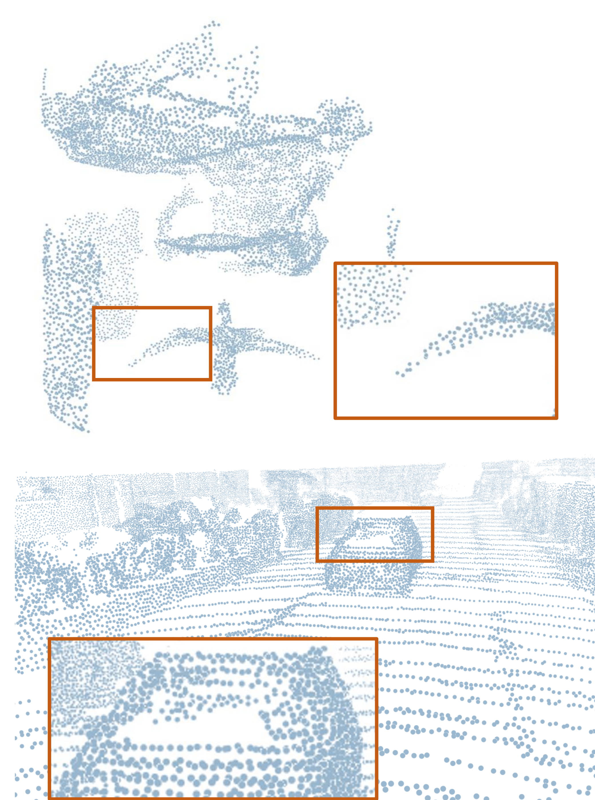
(e) PU-Transformer
