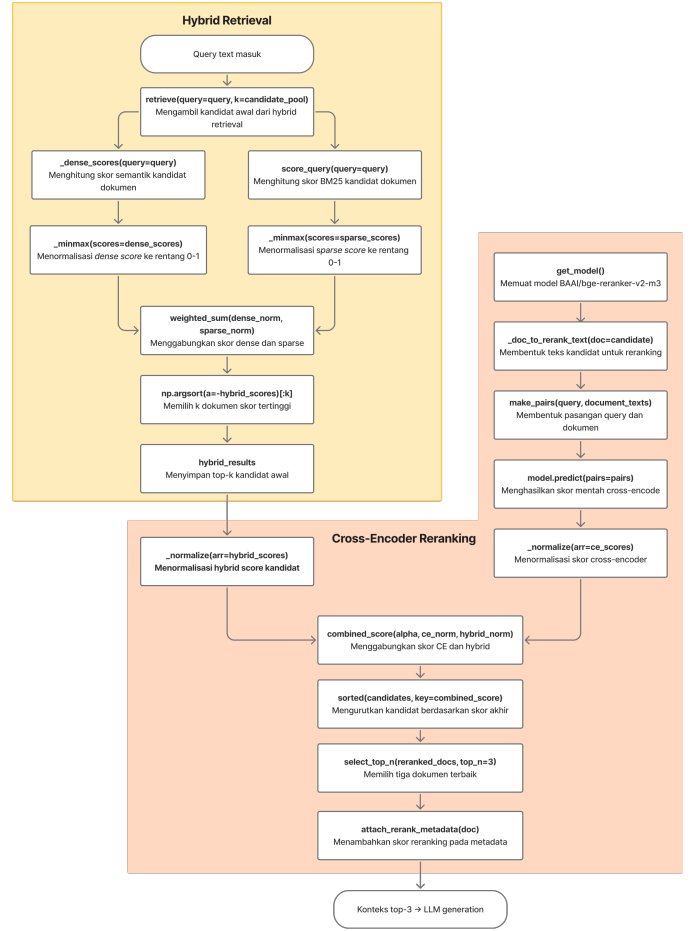
Fig. 2. Cross-encoder reranking pipeline: hybrid retrieval produces a candidate pool, which the cross-encoder re-evaluates before score fusion.
