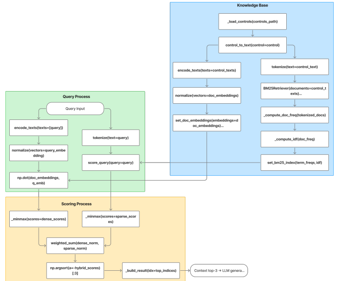
Fig. 1. Hybrid retrieval architecture combining BM25 sparse retrieval with dense embedding retrieval via weighted score fusion.
