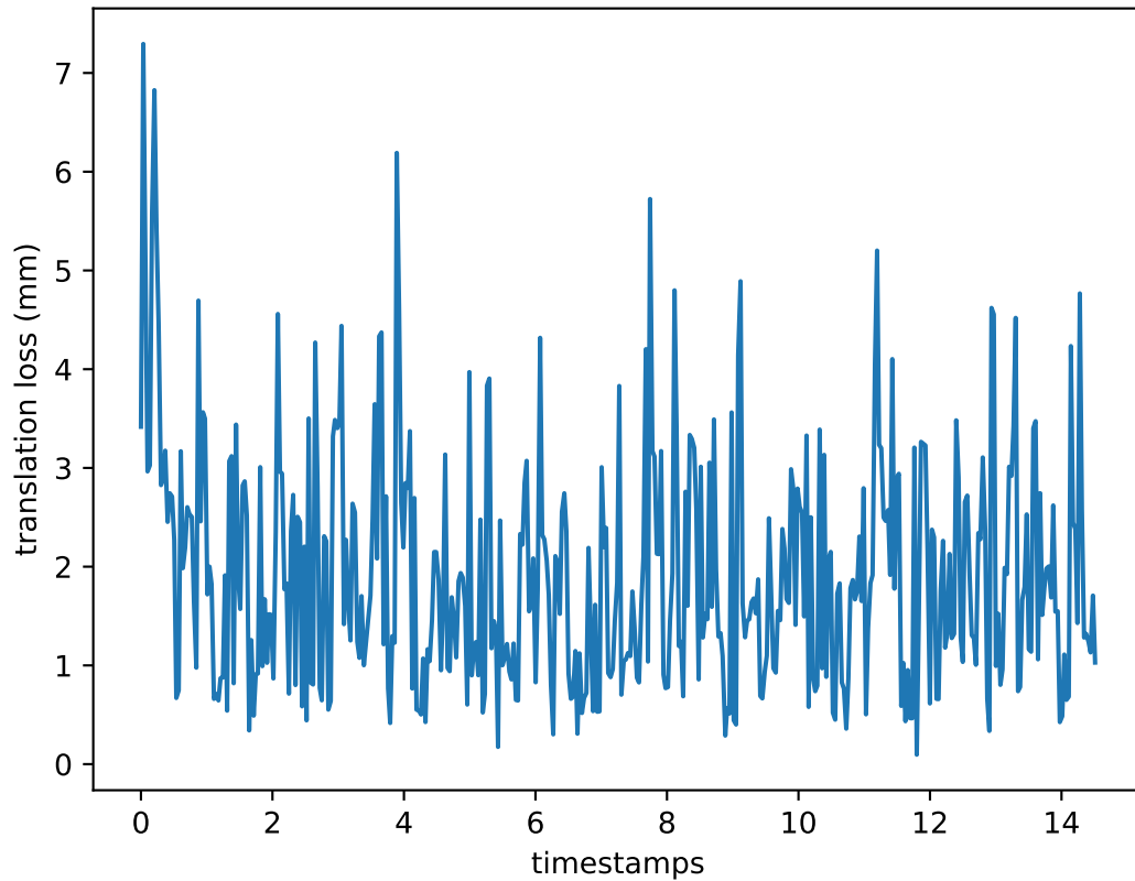
translation loss
