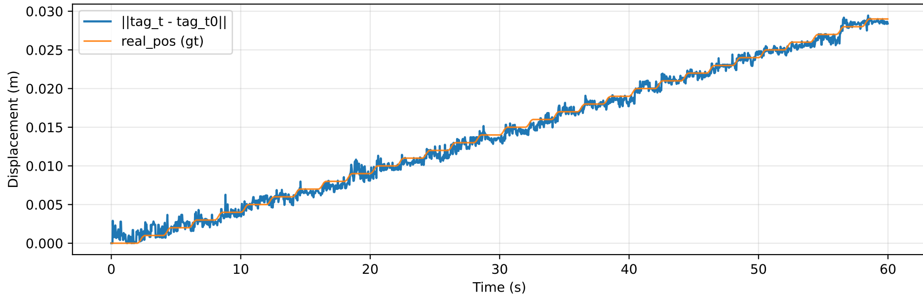
Tag Translation Delta Norm vs GT
