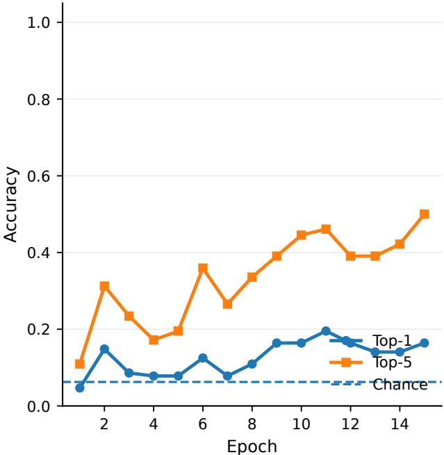
(b) RGB-Thermal Retrieval Accuracy
