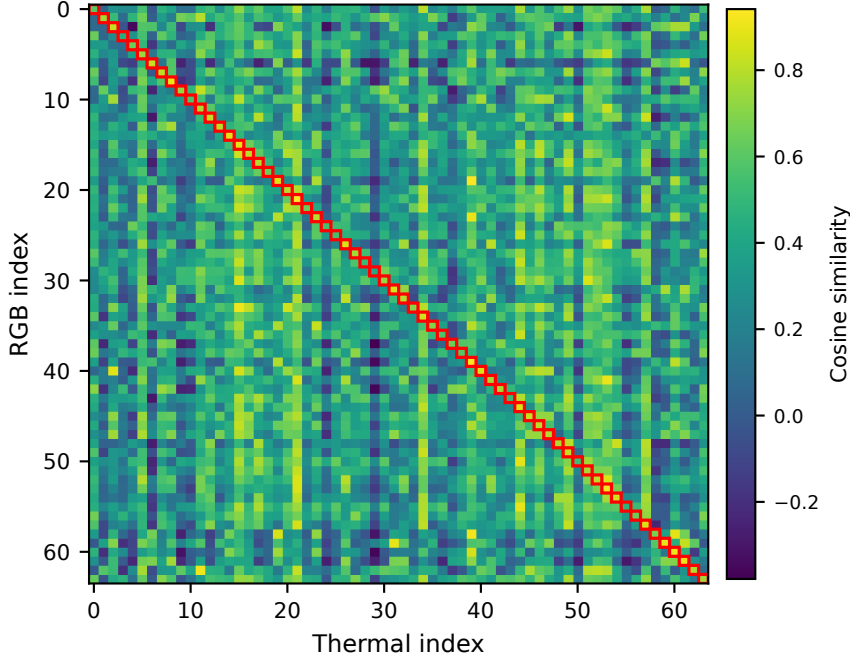
(c) RGB → Thermal Similarity Matrix
