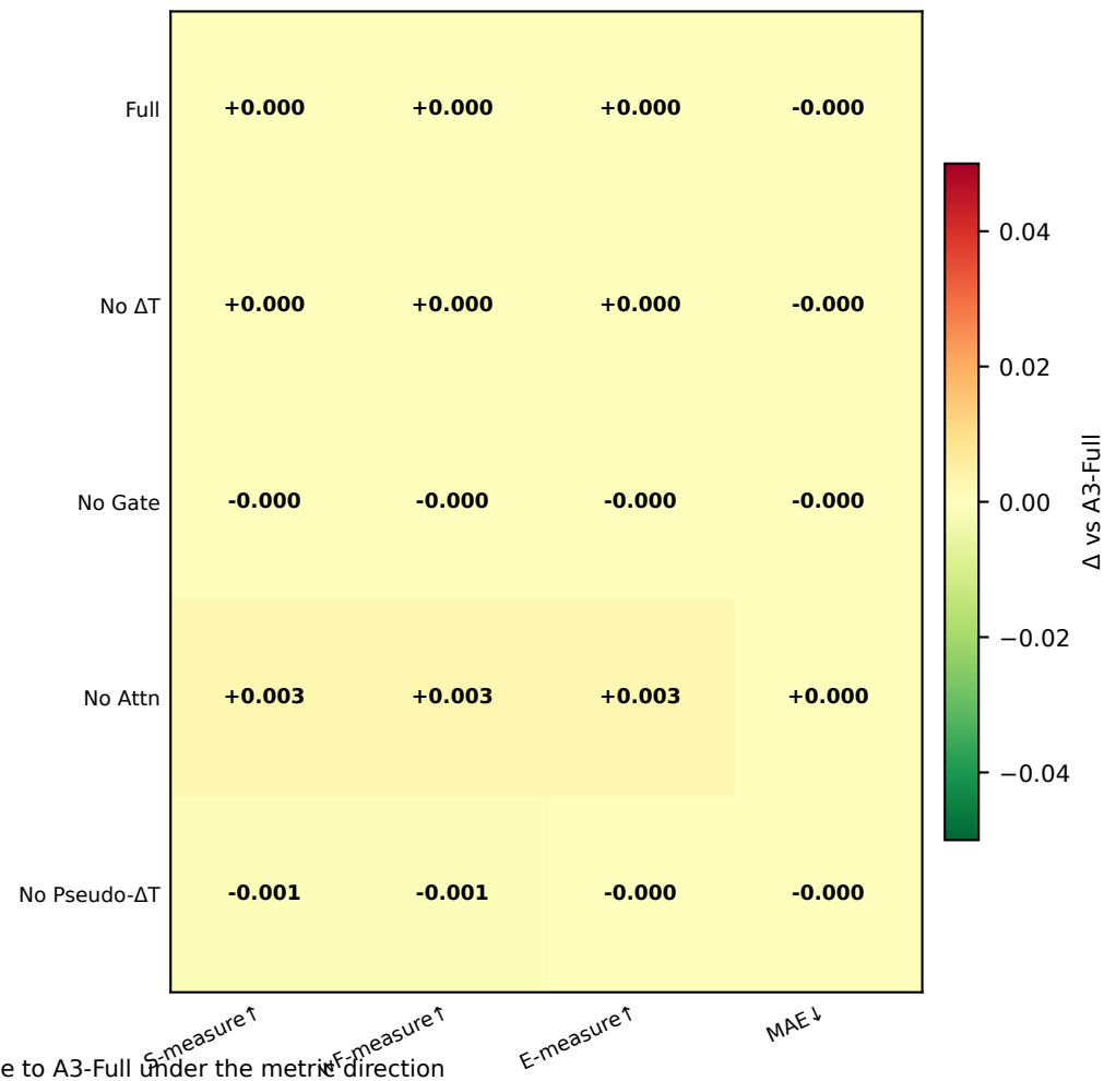
Contribution Relative to A3-Full
