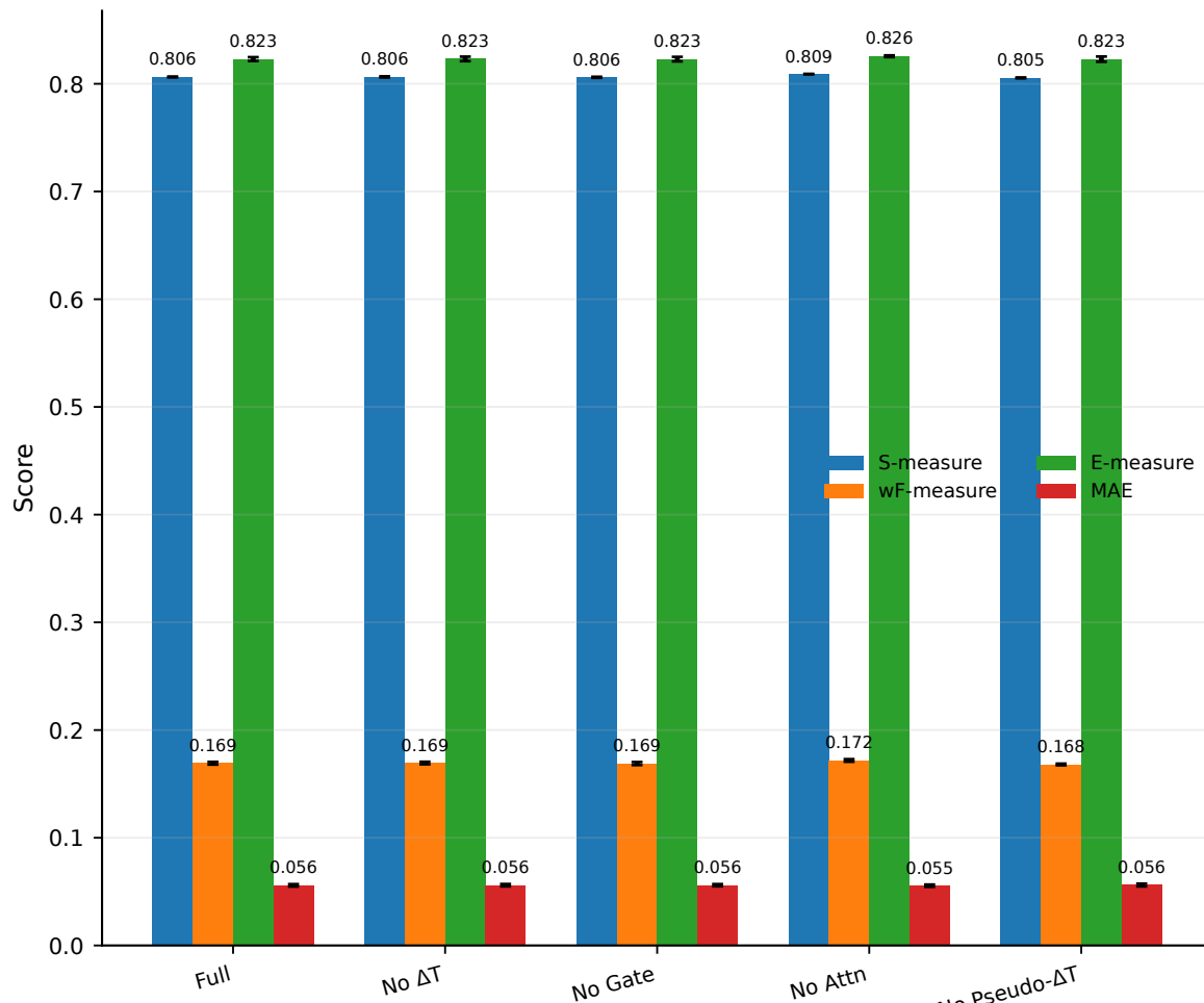
Component Removal — COD10K-test
