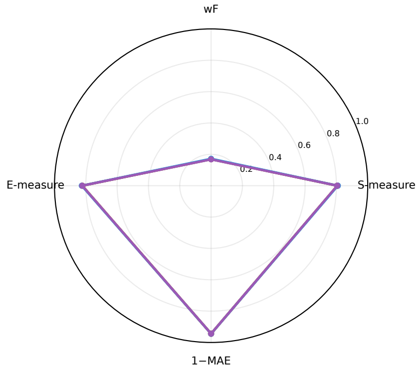
Component Removal
