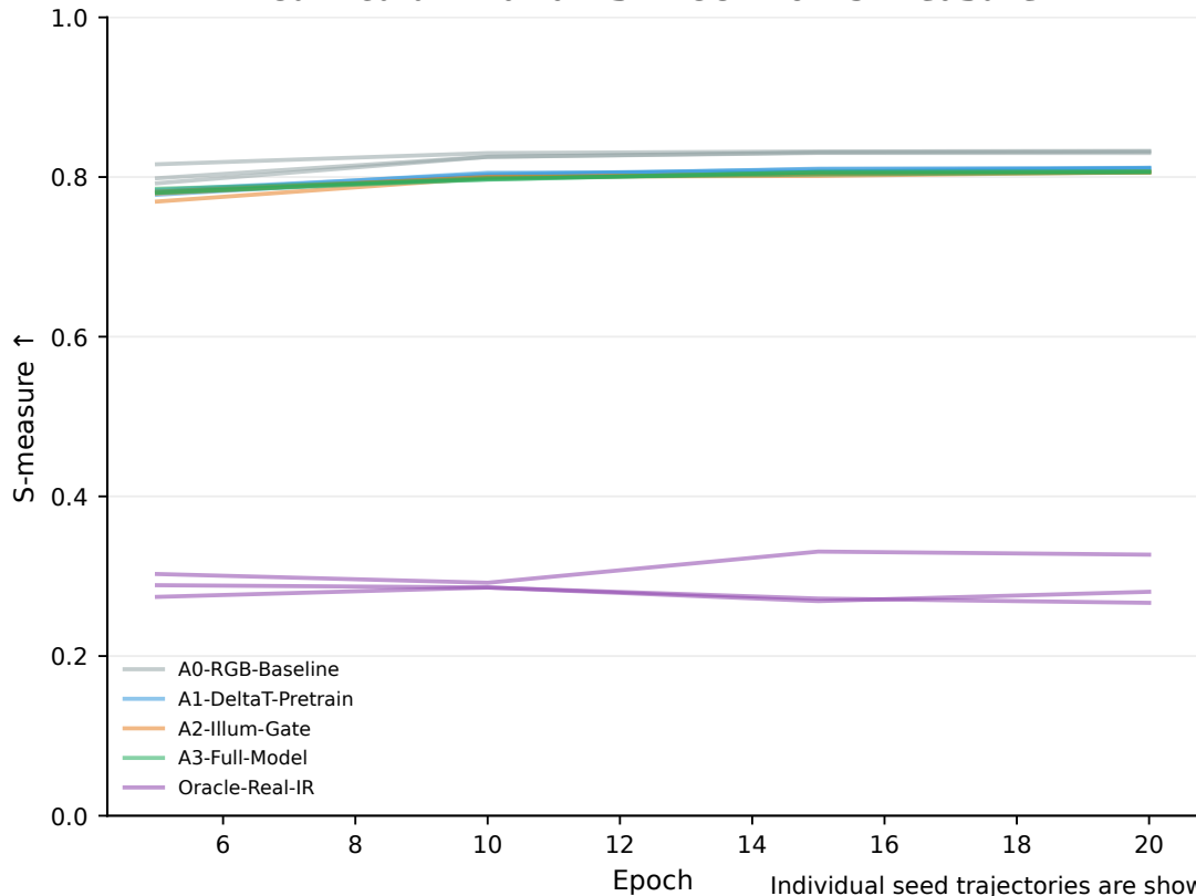
Curriculum Variants — COD10K S-measure
