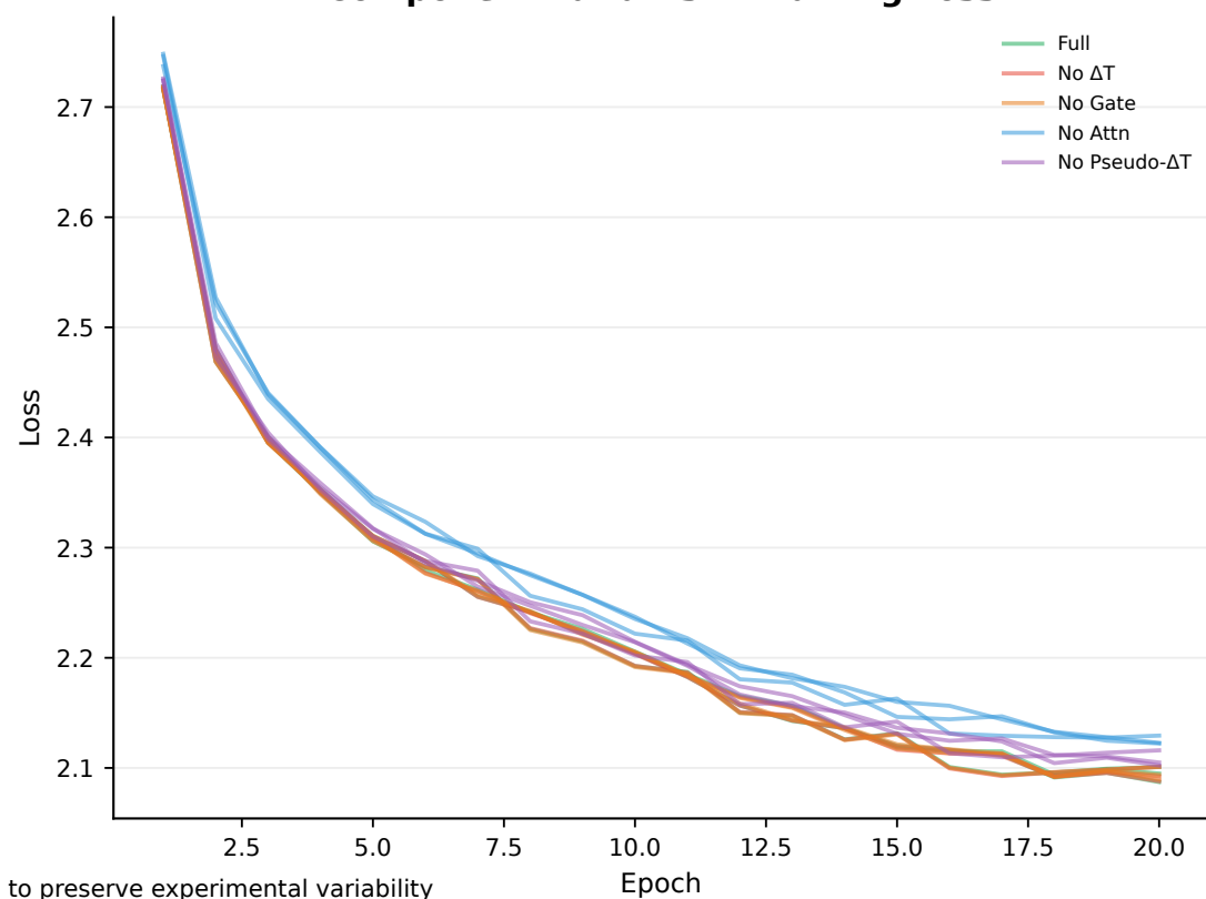
Component Variants — Training Loss
