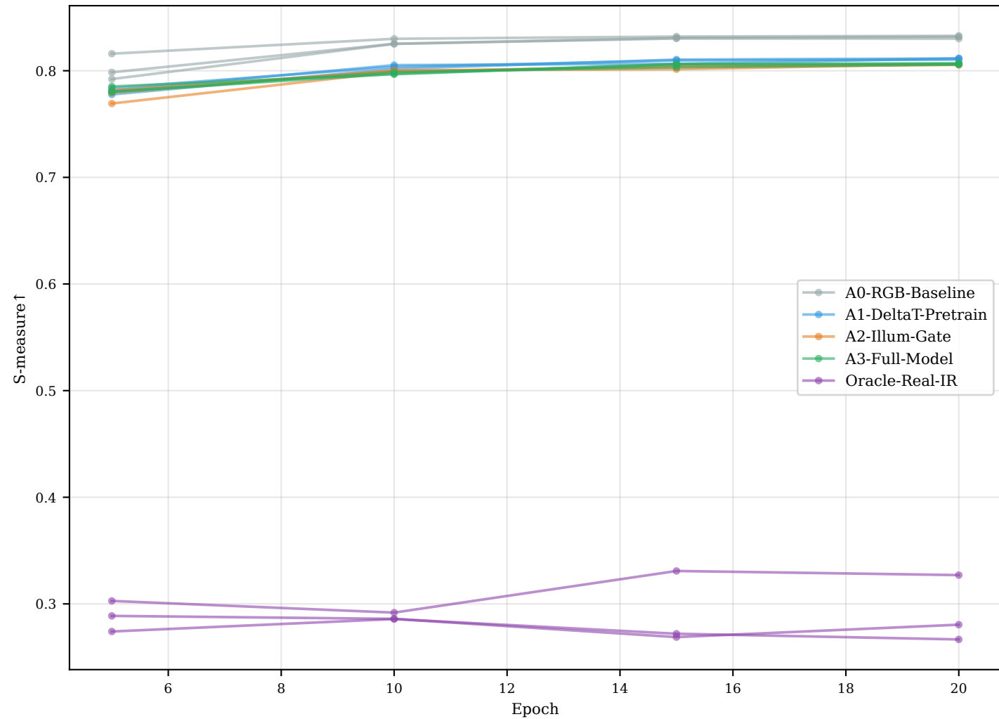
COD10K-test S-measure over Training (3 seeds)
