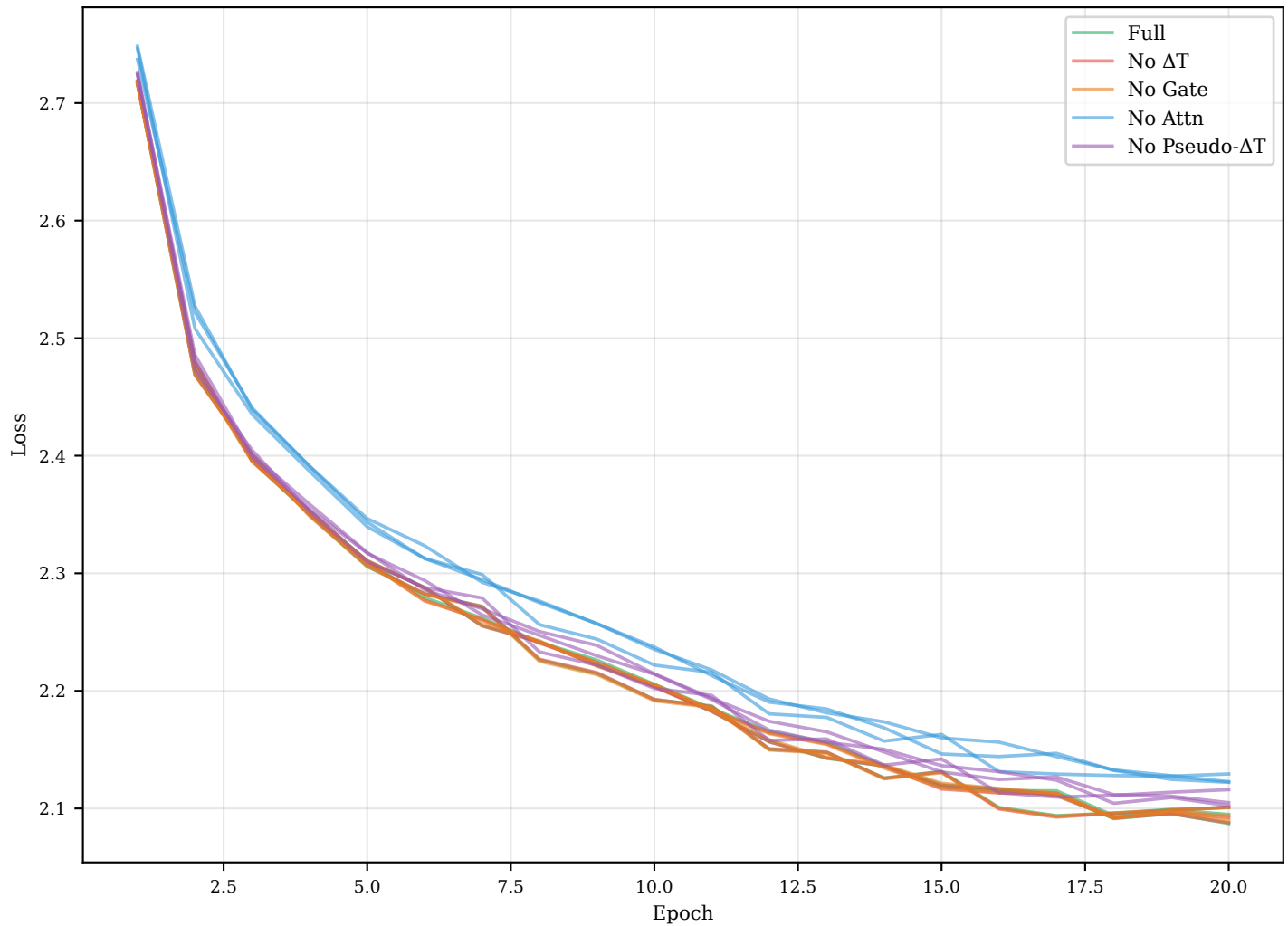
Component Ablation — Training Loss (3 seeds)
