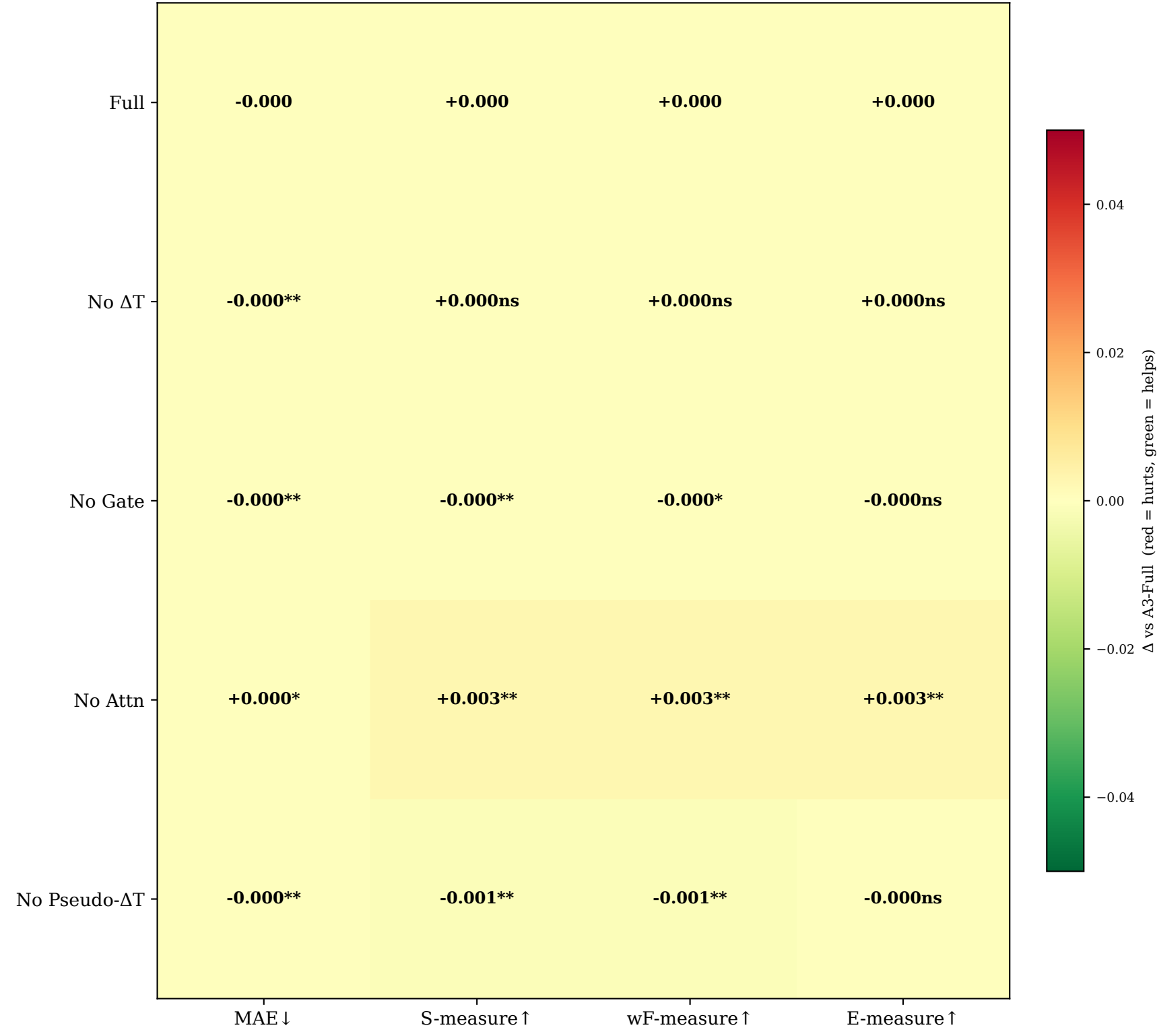
Component Contribution Heatmap Δ vs A3-Full, with significance markers
