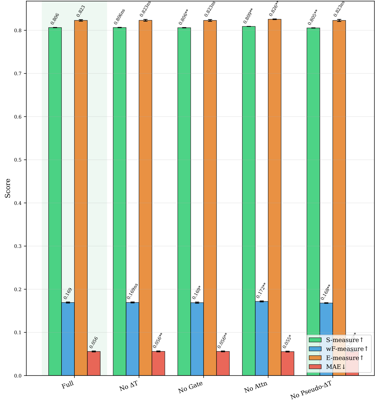
Component Removal — COD10K-test (mean±std/3 seeds; * p<0.05, ** p<0.01, ns=not sig. vs A3-Full)
