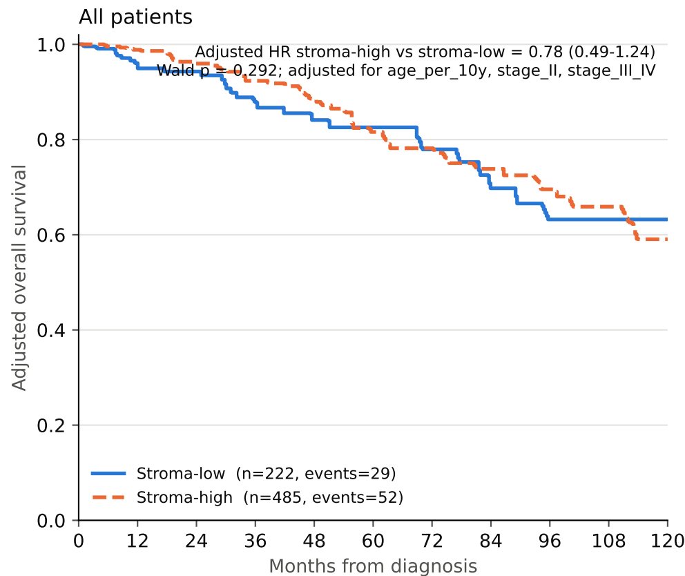
Overall survival by tumor-stroma ratio (stroma-high: ratio < 1) (all patients; censored at 120 months; adjusted for age and stage)
