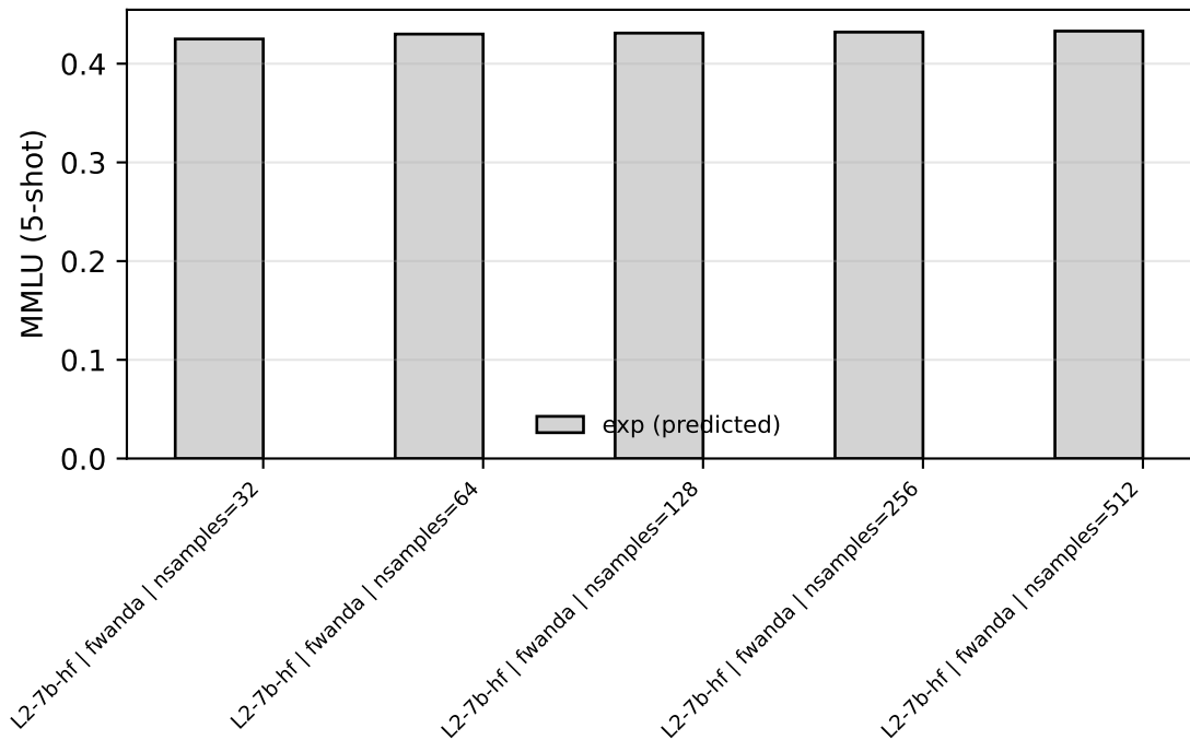
MMLU (5-shot) ( \uparrow better) [ablation_calib_size.csv]
