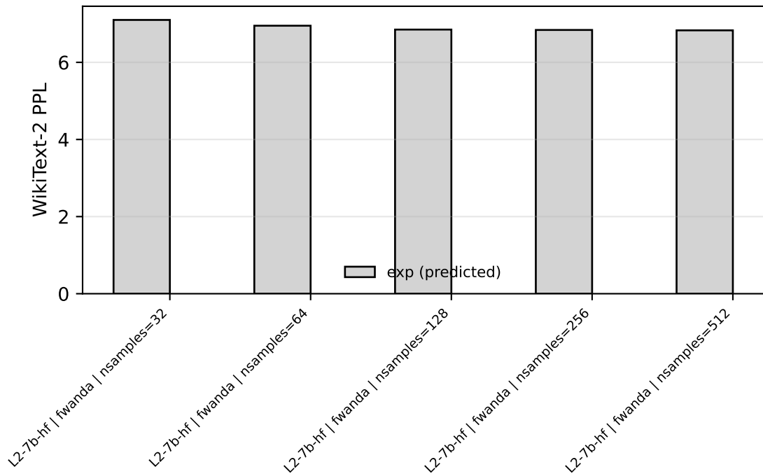
WikiText-2 PPL ( \downarrow better) [ablation_calib_size.csv]
