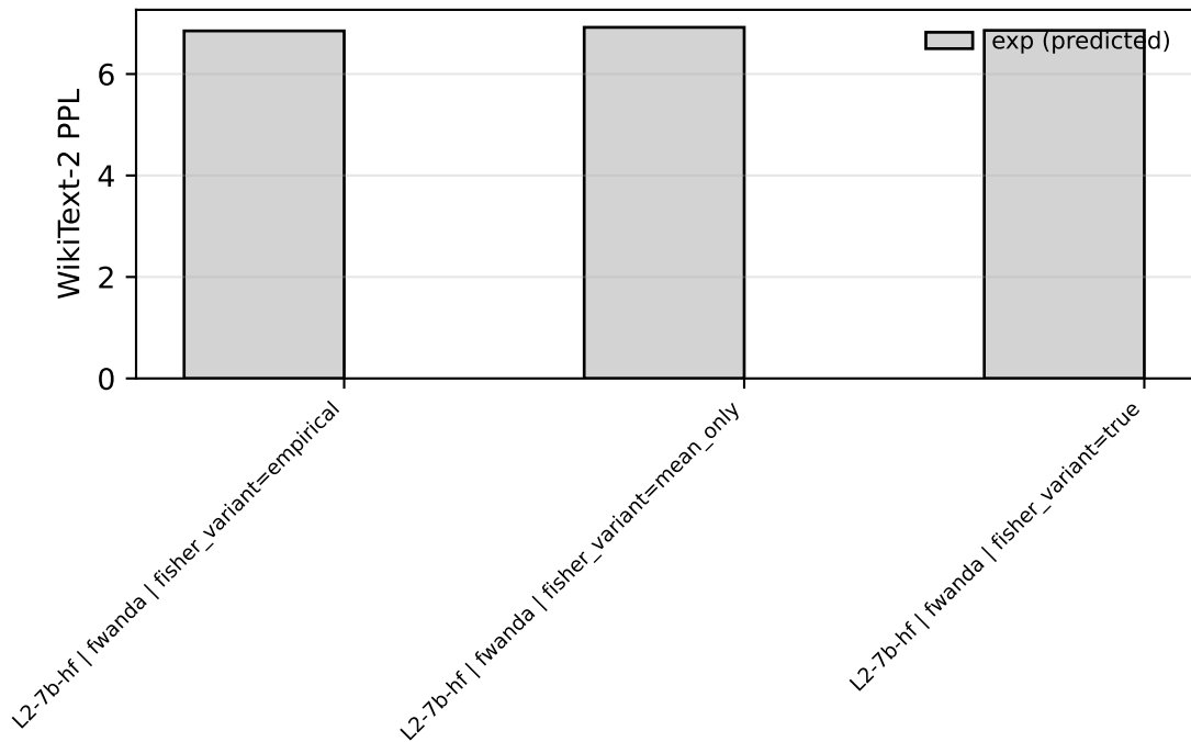
WikiText-2 PPL ( \downarrow better) [ablation_fisher_variants.csv]
