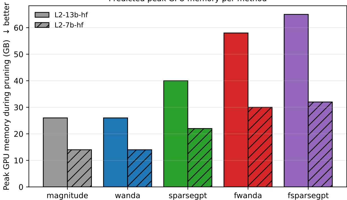
Predicted peak GPU memory per method
