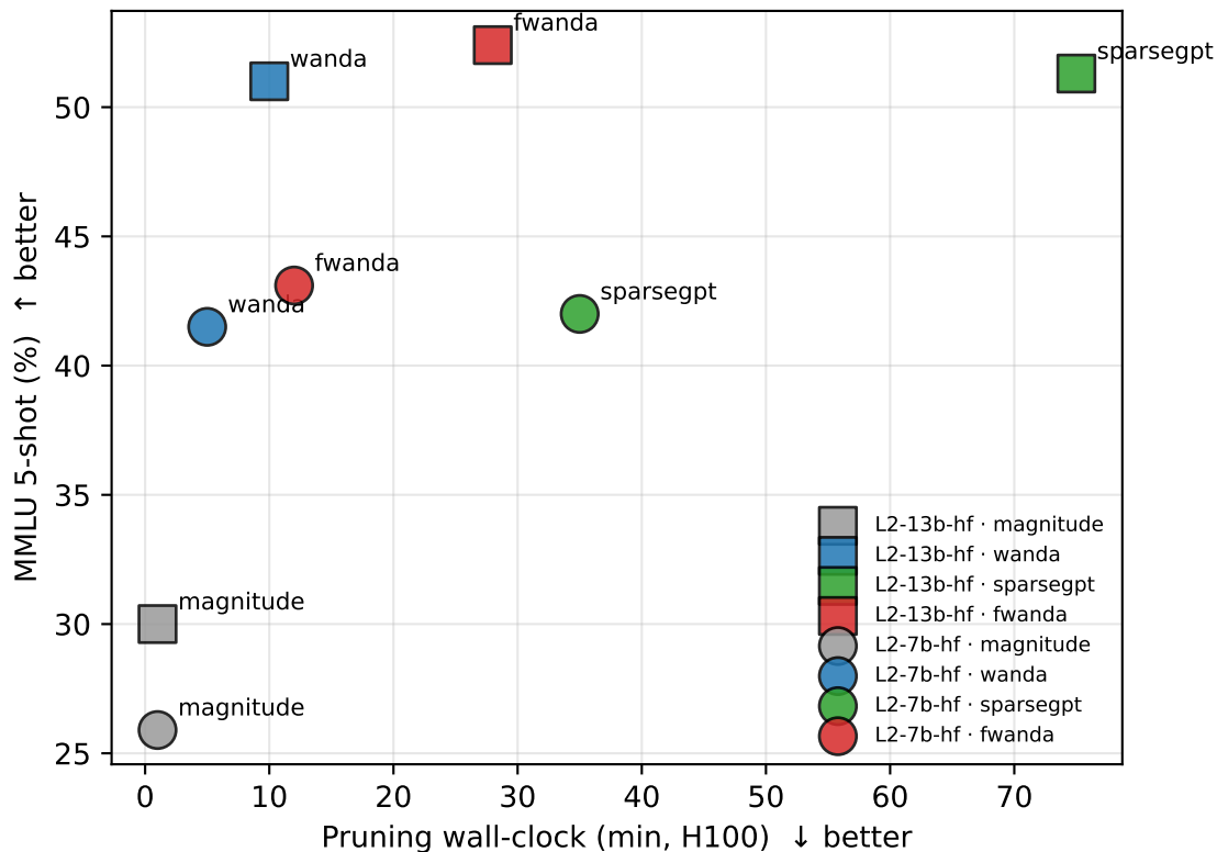
Quality vs. cost (50% unstructured)
